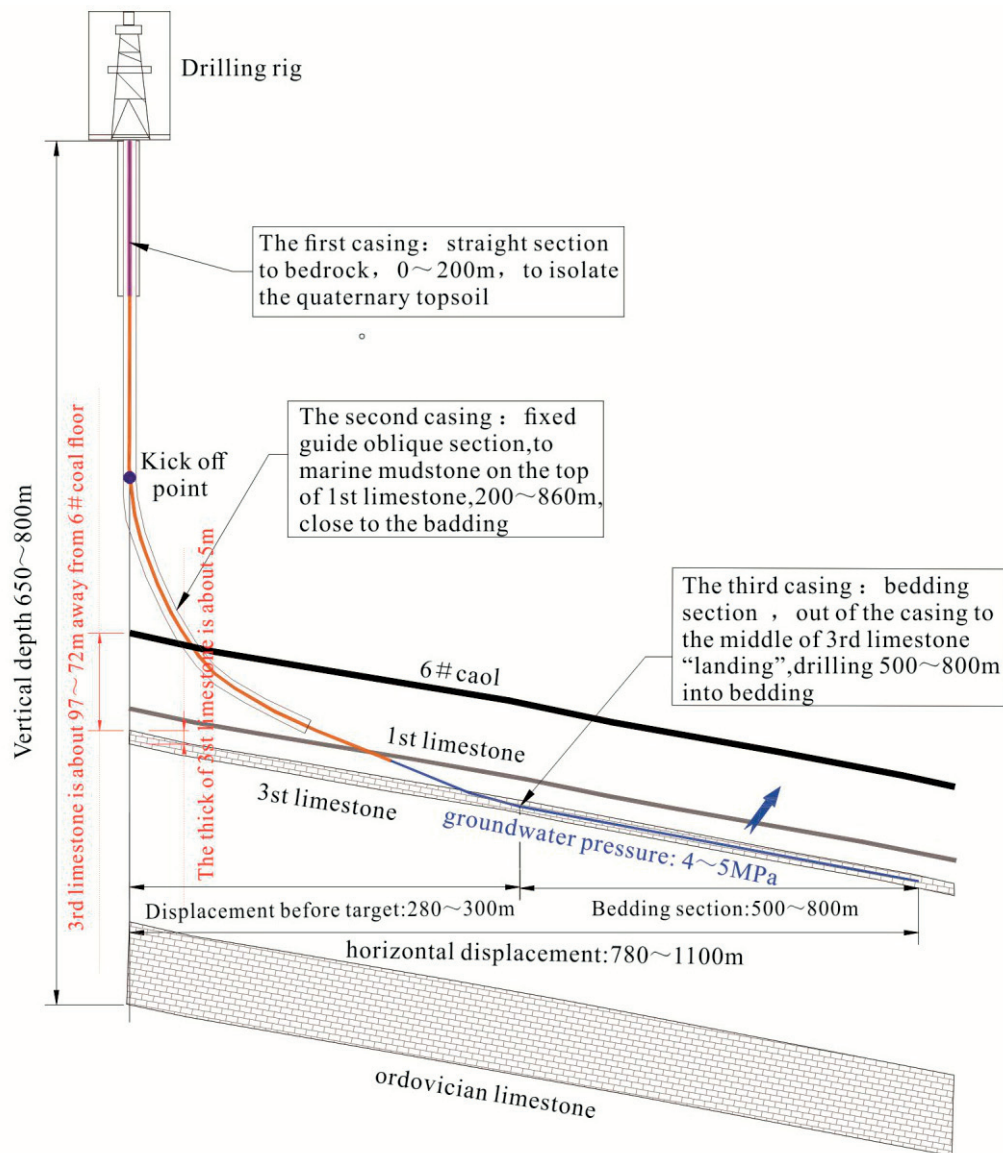
Fig. 1. Profile of surface directional drilling.
