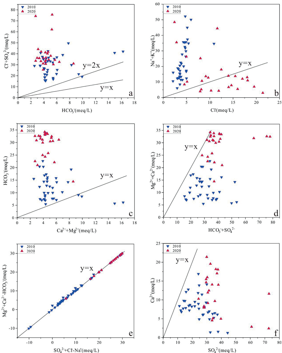
Fig. 8. Proportion diagram of ion combination in the limestone water before and after grouting.
