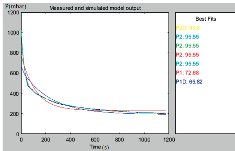
Fig. 8. Pressure simulation identification comparison.
