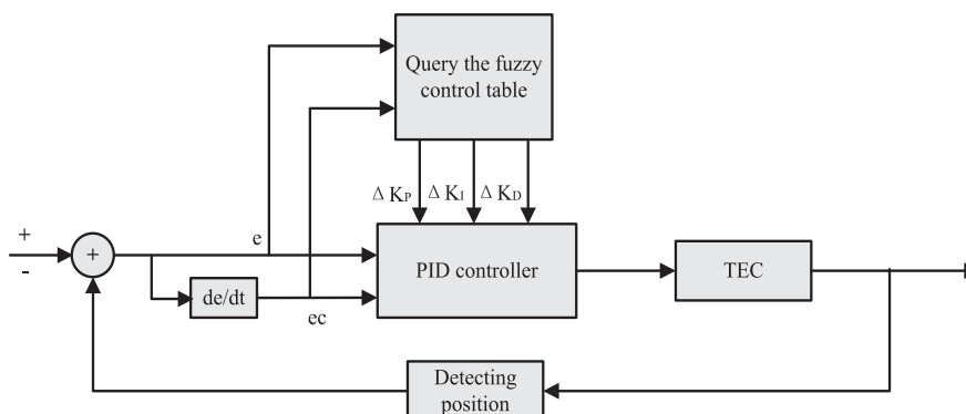
Fig. 9. FA-PID structure block diagram.
