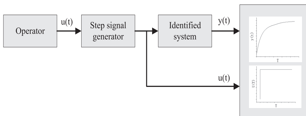
Fig. 4. Schematic diagram of system identification experiment.
