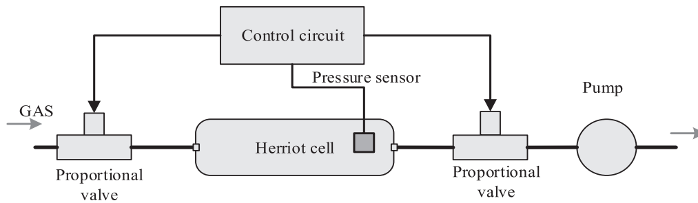
Fig. 7. Pressure control system scheme.
