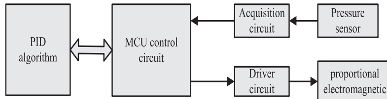
Fig. 3. Schematic diagram of pressure control scheme.
