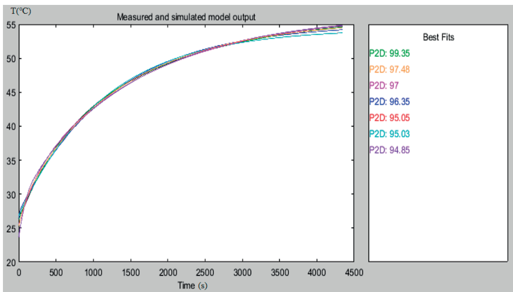
Fig. 6. Comparison of temperature control simulation models.
