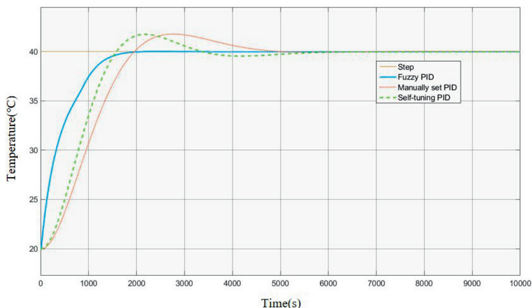
Fig. 12. Simulation results of PID algorithm.
