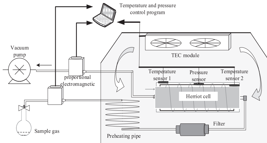
Fig. 1. Overall design block diagram of temperature and pressure control system for laser absorption spectrum measurement.
