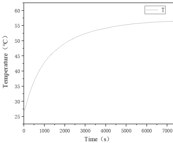
Fig. 5. Step response results of the system.
