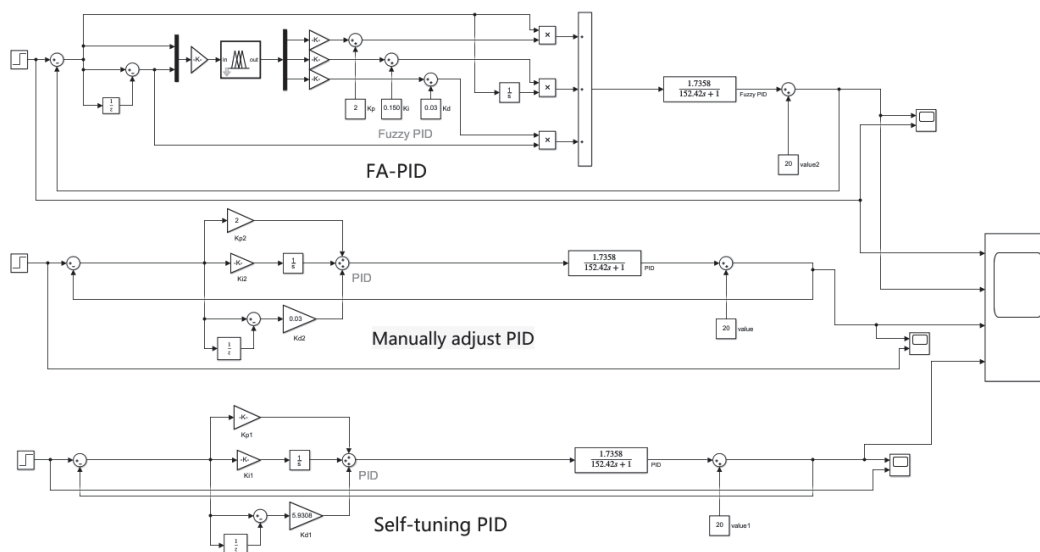
Fig. 11. Matlab simulation model.
