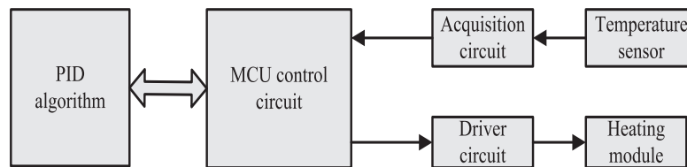
Fig. 2. Schematic diagram of temperature control scheme.
