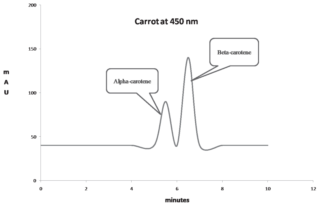
Fig. 3. HPLC-DADchromatogram of Daucus carota L.
