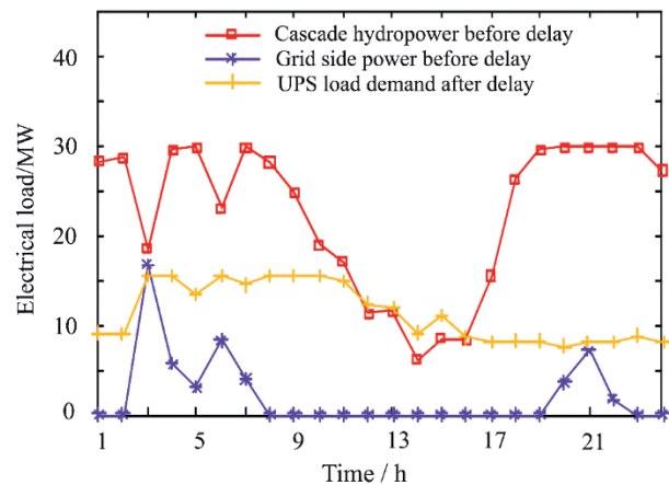
Fig. 4. Scenario 1 output of cascade hydropower, power grid and data center power consumption.
