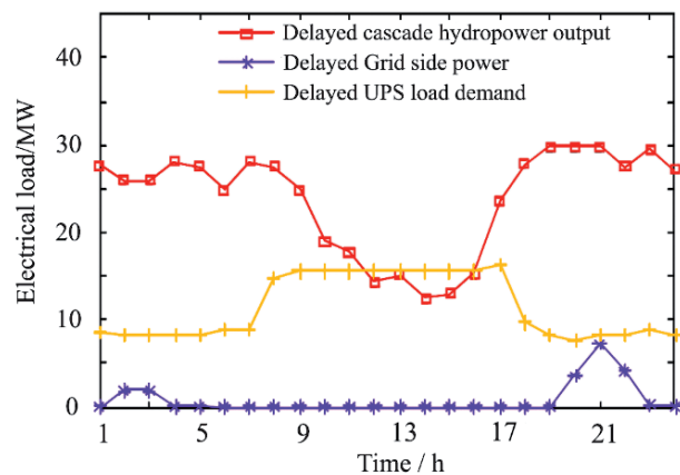
Fig.5. Scenario 2 output of cascade hydropower, power grid and data center power consumption.
