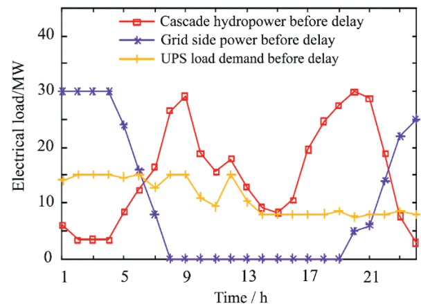
Fig. 7. Scenario 5 output of cascade hydropower, smart grid and data center consumption.
