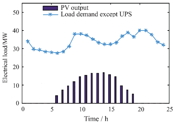
Fig. 6. Scenarios 5 and 6 output of solar and load side demand.
