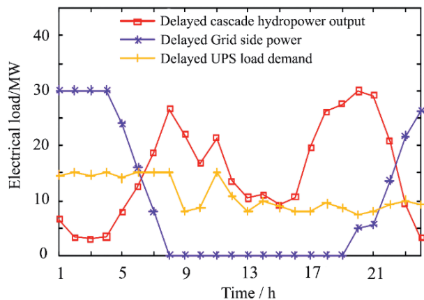
Fig. 8. Scenario 6 output of cascade hydropower, smart grid and data center consumption.
