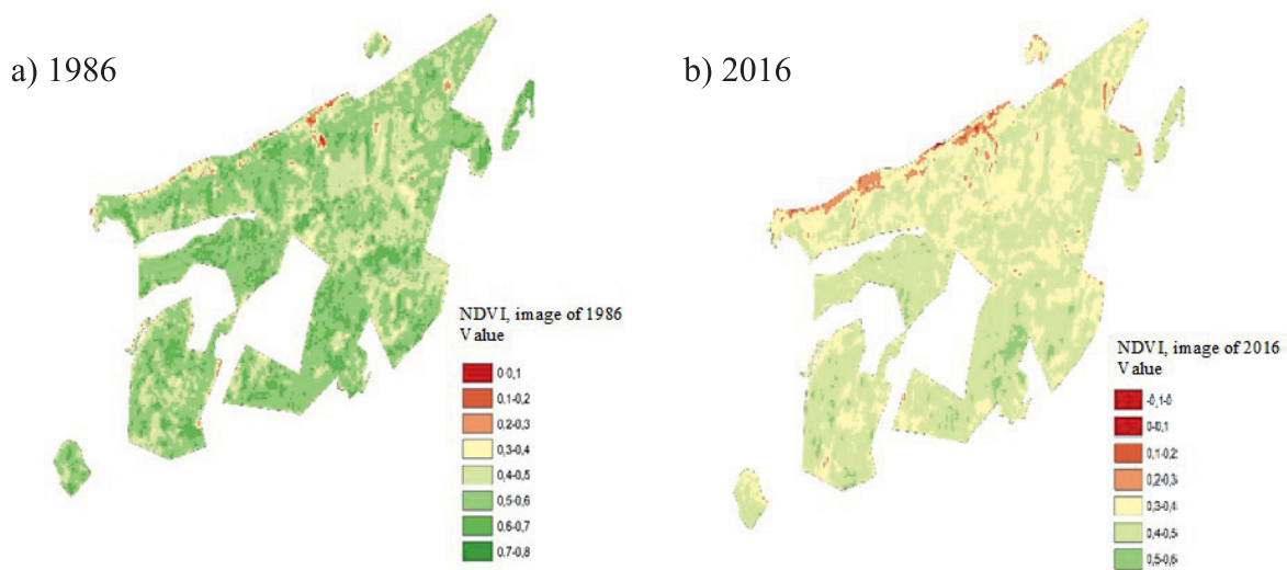
Fig. 4. NDVI index in various years.
