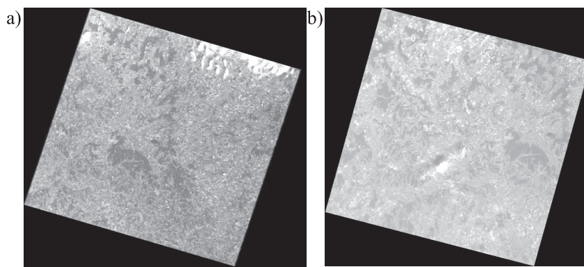
Fig. 3. Satellite images used to calculate the NDV index. a) image taken in 1986 by Landsat-5 satellite; b) image taken in 2016 by Landsat-8 satellite.
