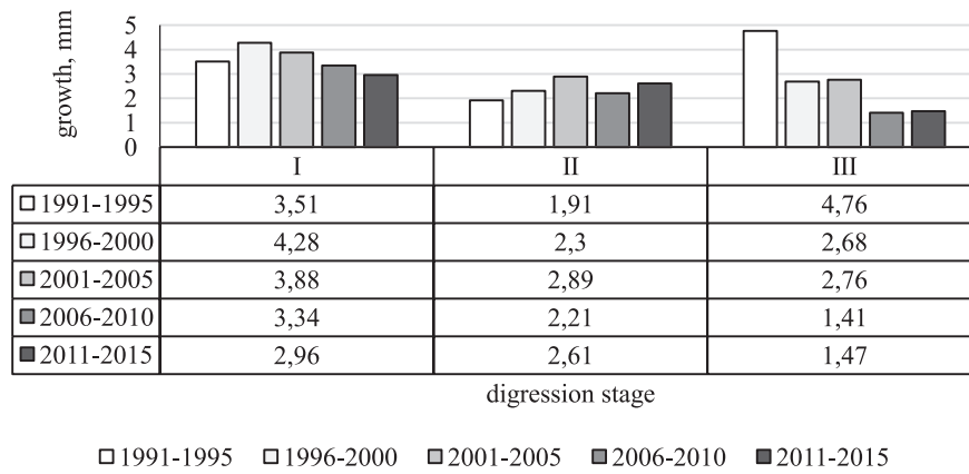
Fig. 2. Dynamics of radial increment depending on stages of poplar recreational Digression.
