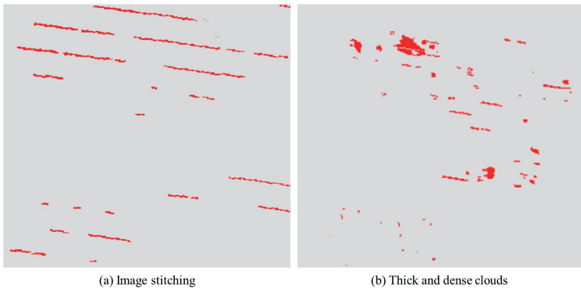
Fig. 6. Forest disturbance over-detection areas in Jilin Province.
