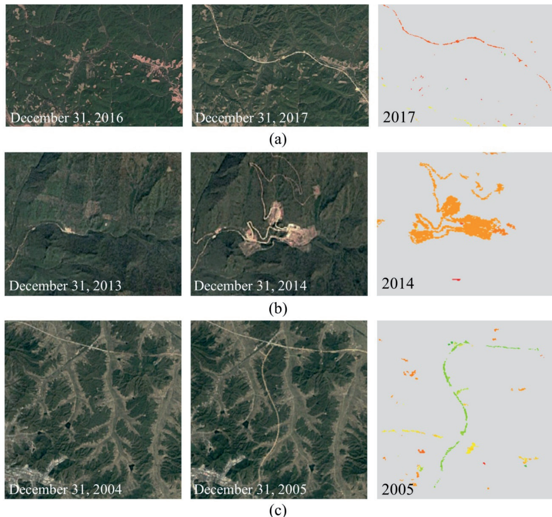
Fig. 2. Results of local forest dynamics change detection in Jilin Province.
