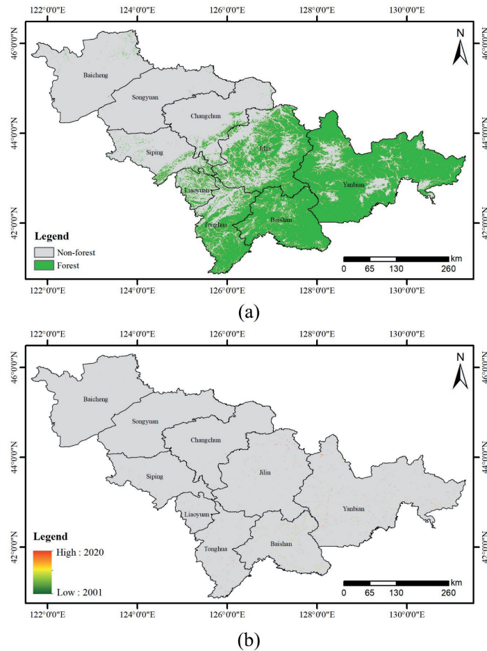
Fig. 3. a) Spatial distribution of the Globeland30 forest union for 2000 and 2020 in Jilin Province; b) Spatial and temporal distribution of changes in forest dynamics in Jilin Province from 2000 to 2020.
