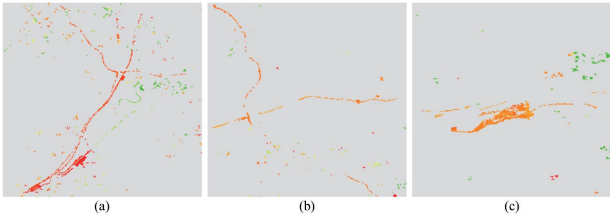
Fig. 5. Conversion of forests to construction land.
