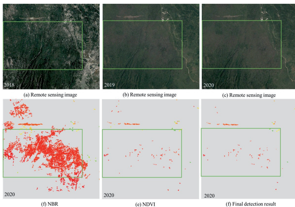
Fig. 7. Forest disturbance detection results for different indexes.
