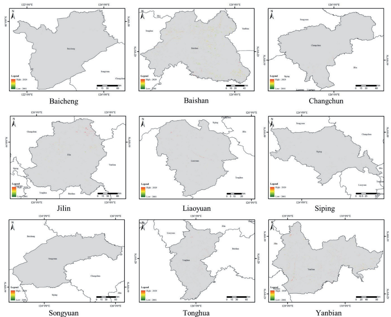
Fig. 4. Spatial and temporal distribution of changes in forest dynamics in prefecture-level cities of Jilin Province from 2000 to 2020.
