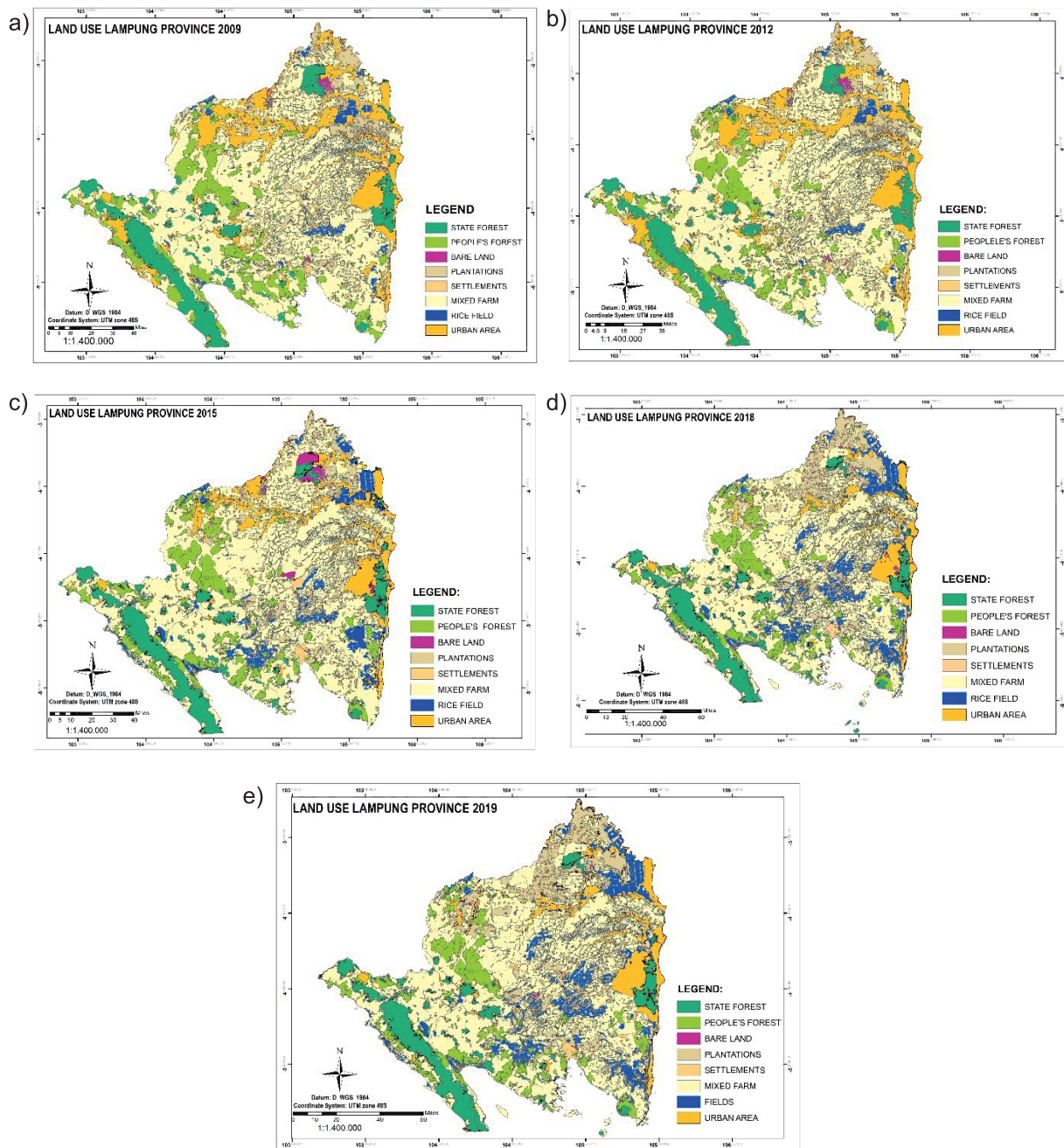
Fig. 2. Land use of Lampung Province (Source Landsat Interpretation accompanied by field ground checking of a) 2009, b) 2012, c) 2015, d) 2018, and e) 2019 after [5].
