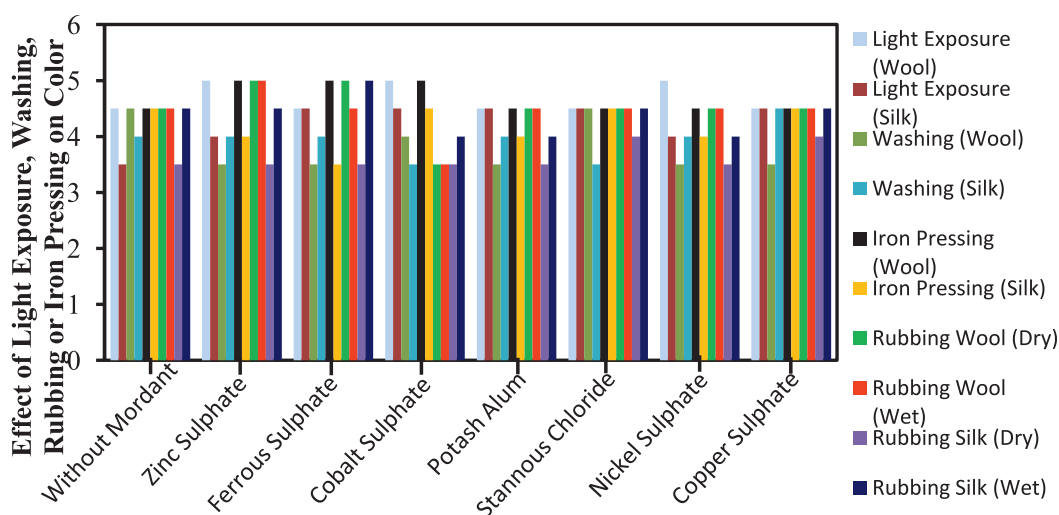
Fig. 1. Graphical representation of color change upon light exposure, washing, rubbing or iron pressing of dyed cloth.
