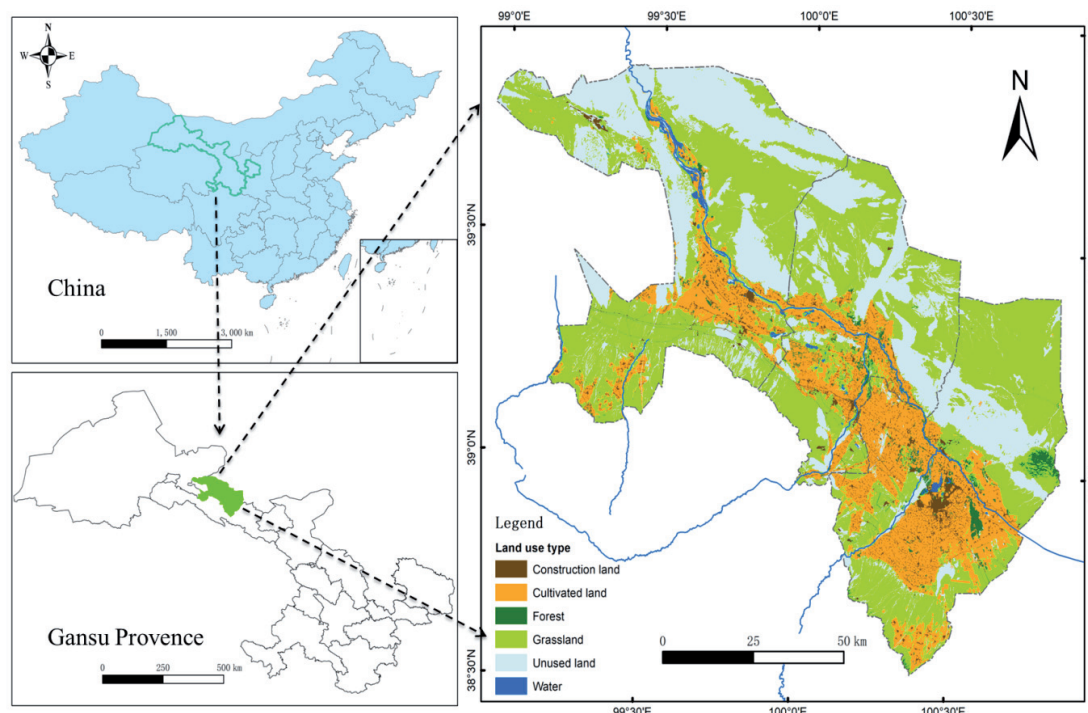
Fig. 1. Location of the middle reaches of the Heihe River Basin [21].
