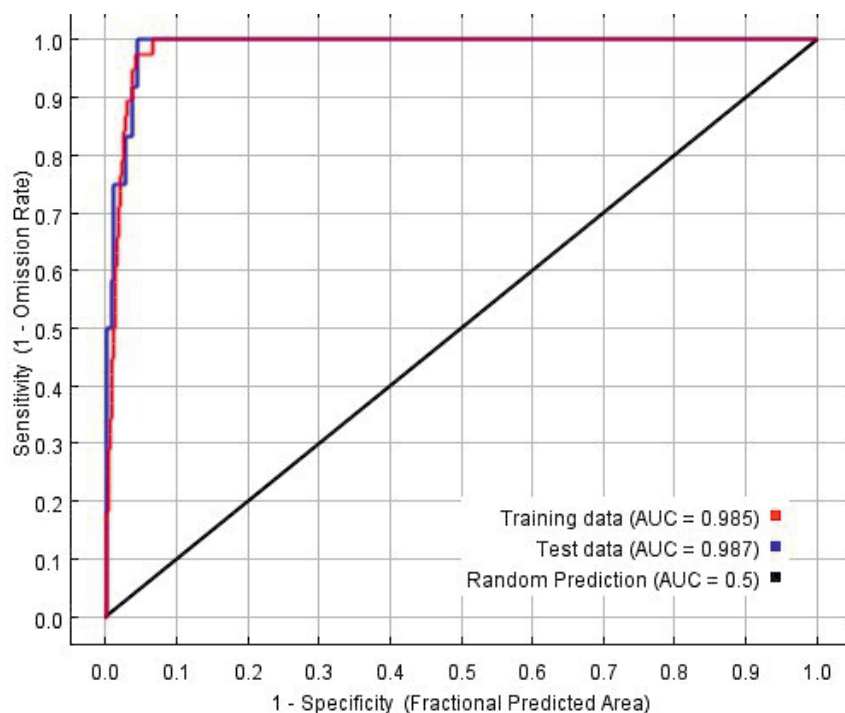
Fig. 3. Receiver operating characteristic curve of P. rockii Maxent model.
