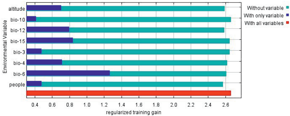
Fig. 4. The jackknife test result of environmental factor for P. rockii .
