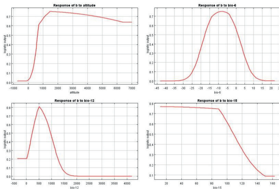
Fig. 5. Response curves of existence probability of P. rockii .
