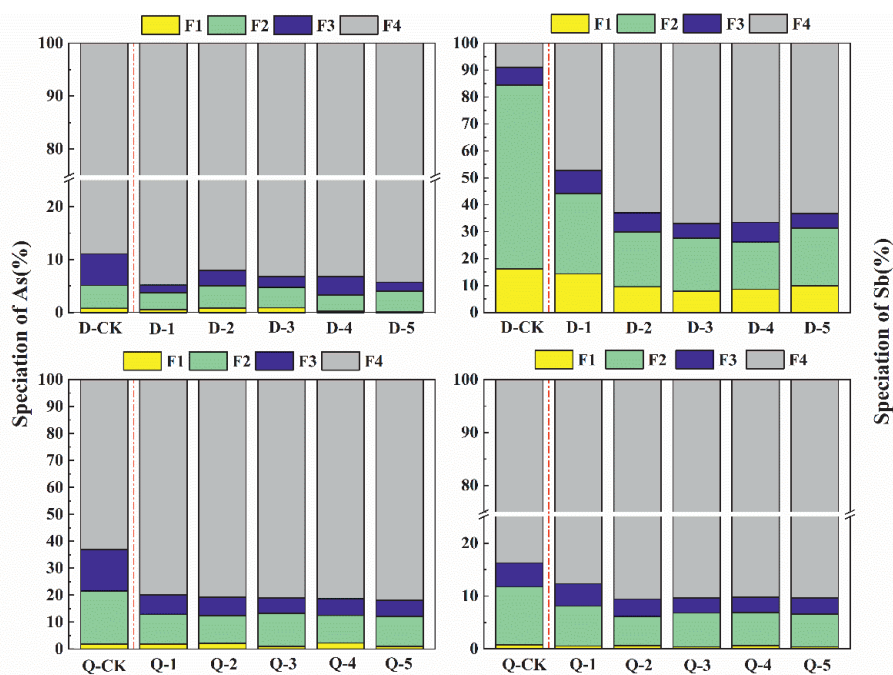
Fig. 4. Morphological transformation of As and Sb in Du Shan and Qing Long antimony mine before and after stabilization.
