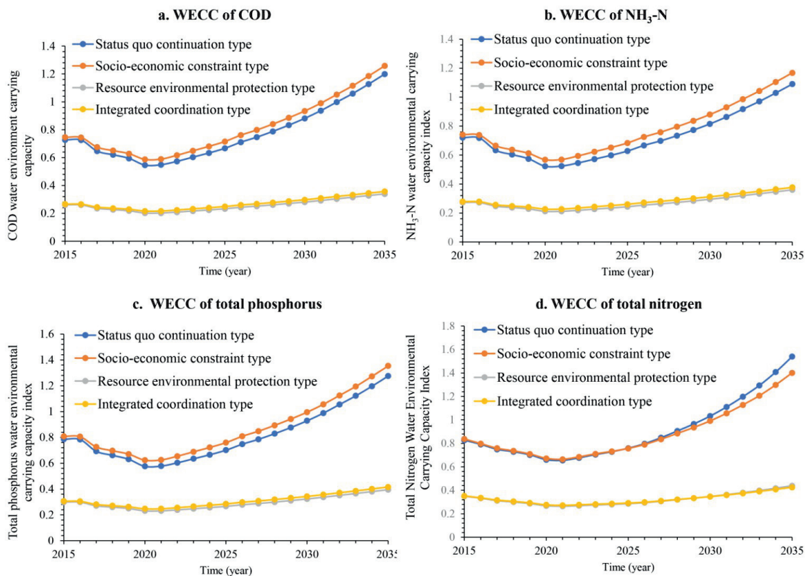
Fig. 6. Simulation results of water environment carrying capacity in the Tongyang River Basin under different scenarios.
