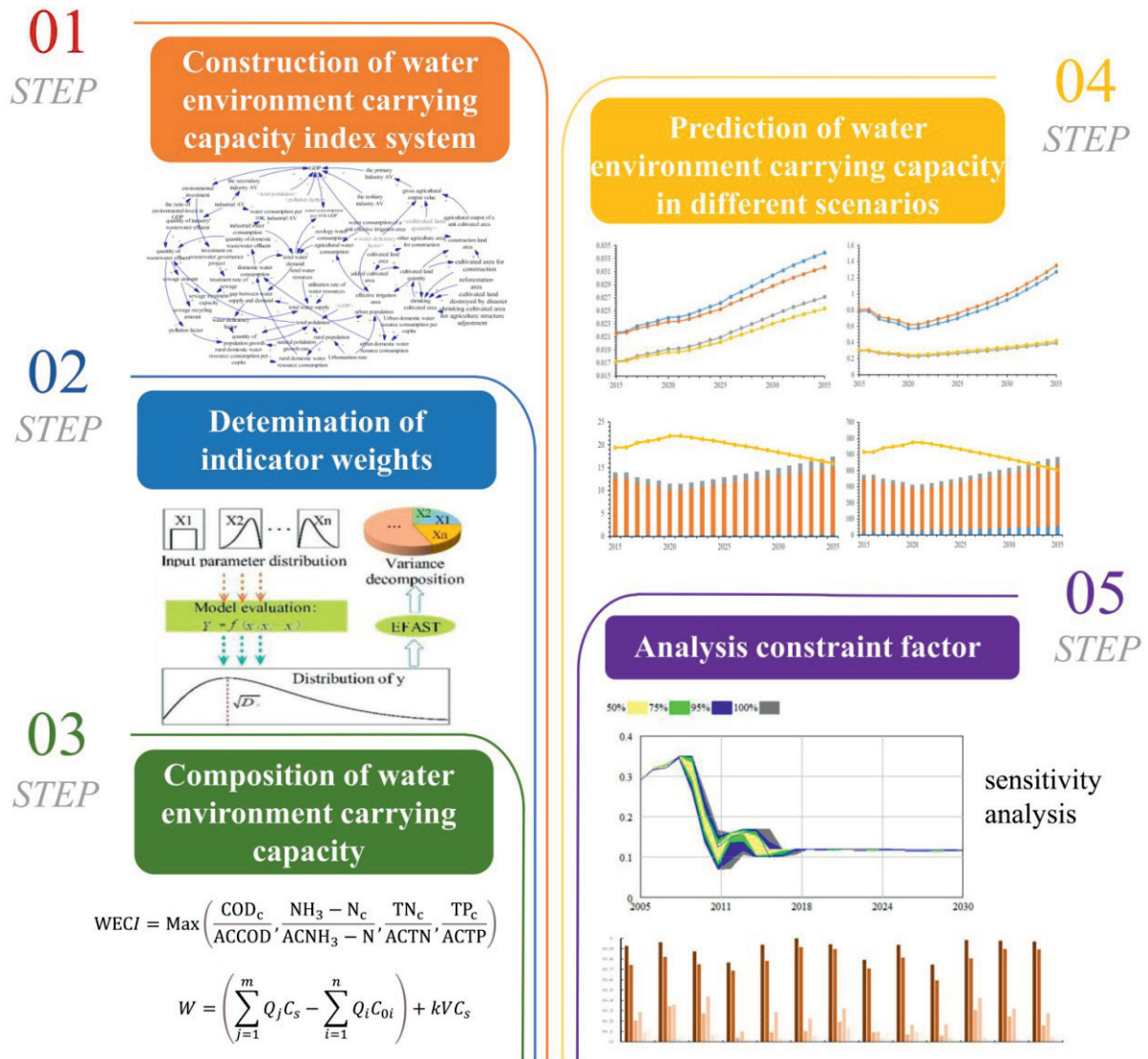
Fig. 2. Flow chart of water environmental carrying capacity (WECC) simulation.
