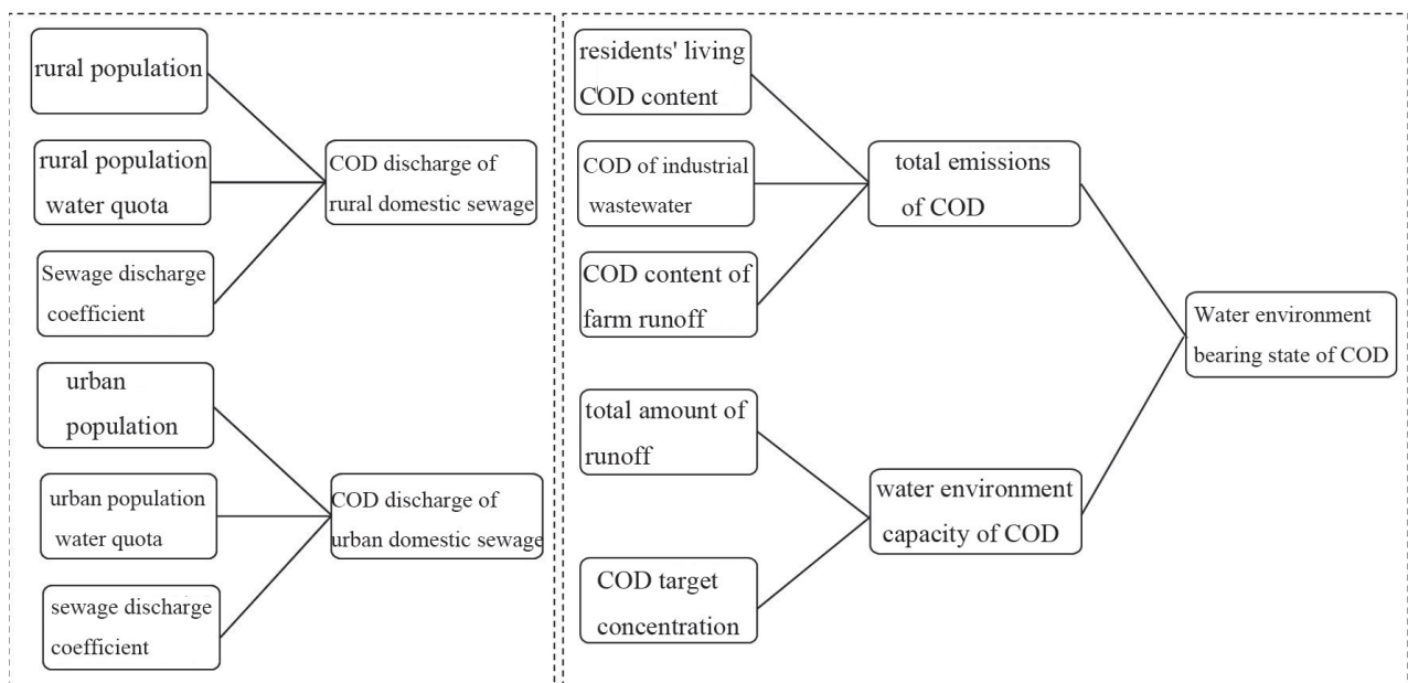
Fig. 3. Regulation mechanism of chemical oxygen demand (COD) carrying capacity.
