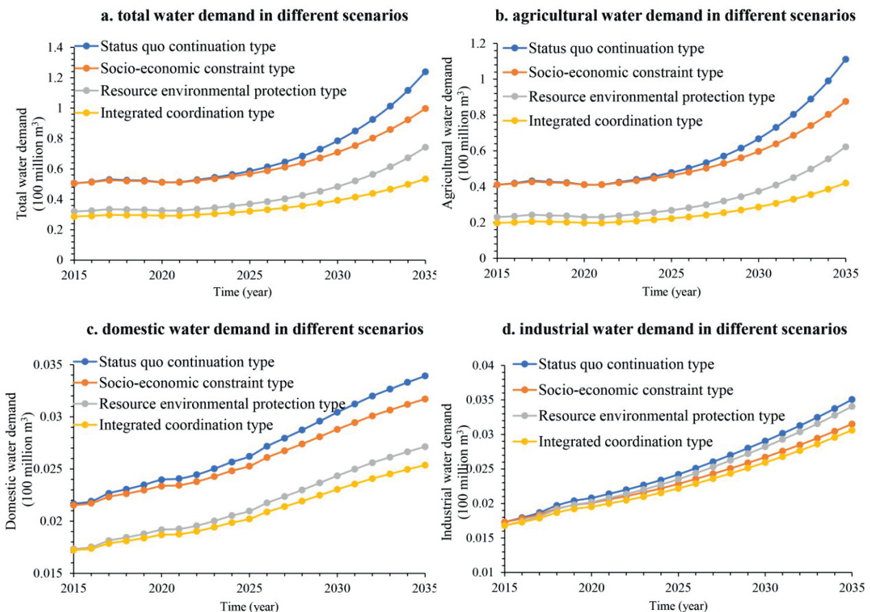
Fig. 5. Simulation results of production and domestic water demand under different scenarios.
