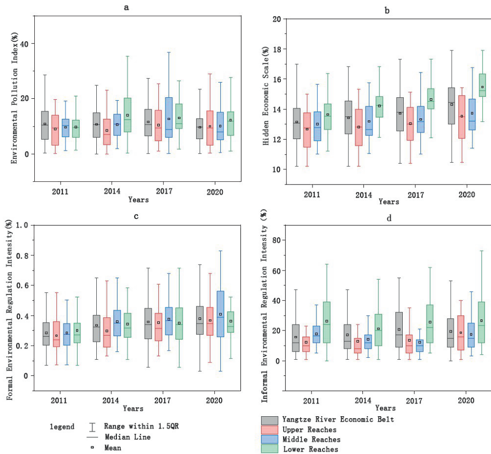
Fig. 2. Box plots of changes in the hidden economic scale, environmental regulation intensity, and environmental pollution index in the YREB in 2011, 2014, 2017 and 2020.
