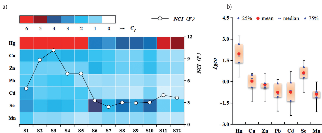
Fig. 3. The C_p , I_{geo} , and NCI(F) values of heavy metals in the study area.
