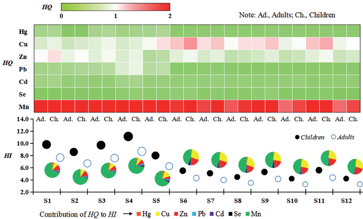
Fig. 6. Non-carcinogenic risk of the seven heavy metals for children and adults in the study area. Note: Hazard Quotient ( HQ ) values (a), Hazard Index ( HI ) values (b, black-white circle figure), and the contribution of HQ/HI (b, pie chart).
