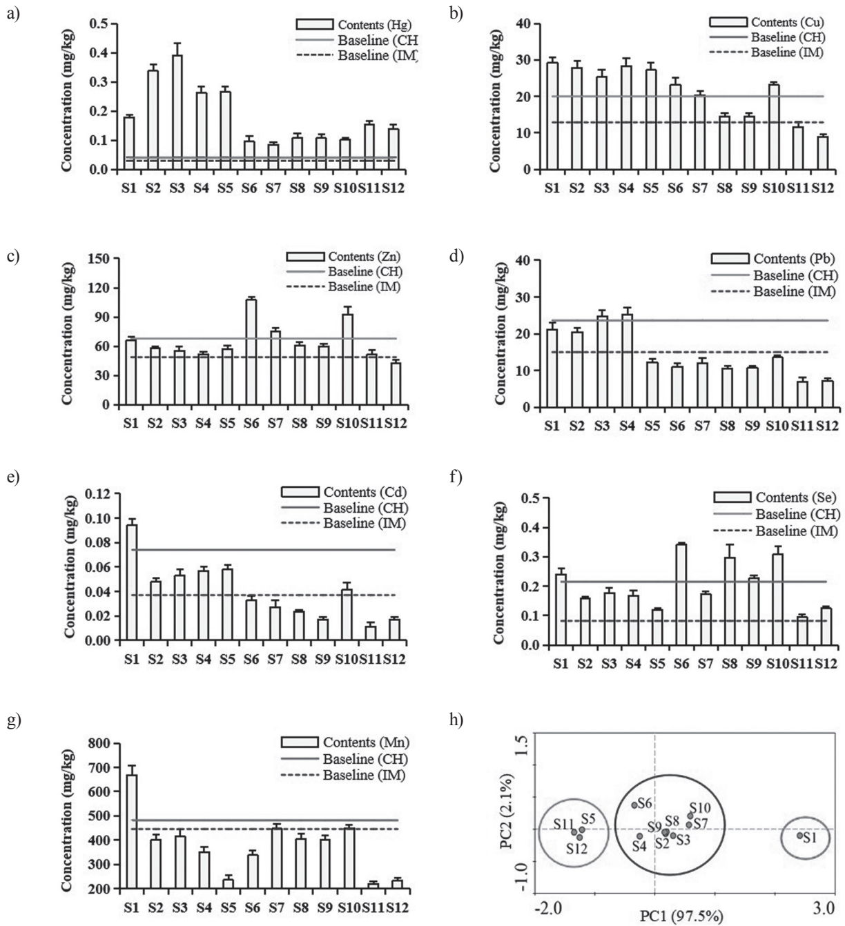
Fig. 2. The content of heavy metals in the soils and results of principal component analysis (PCA) based on the contents of seven heavy metals in each soil sample.
