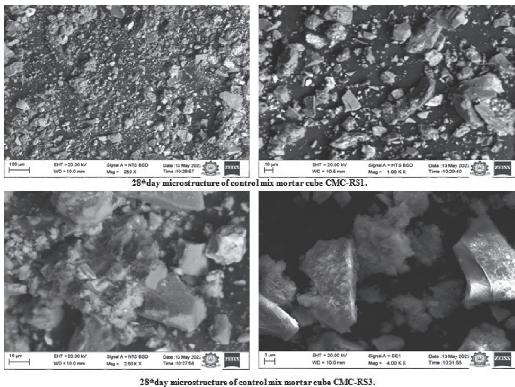
Fig. 3 Microstructure of control mix mortar cubes (CMC-RS1 and CMC-RS3).
