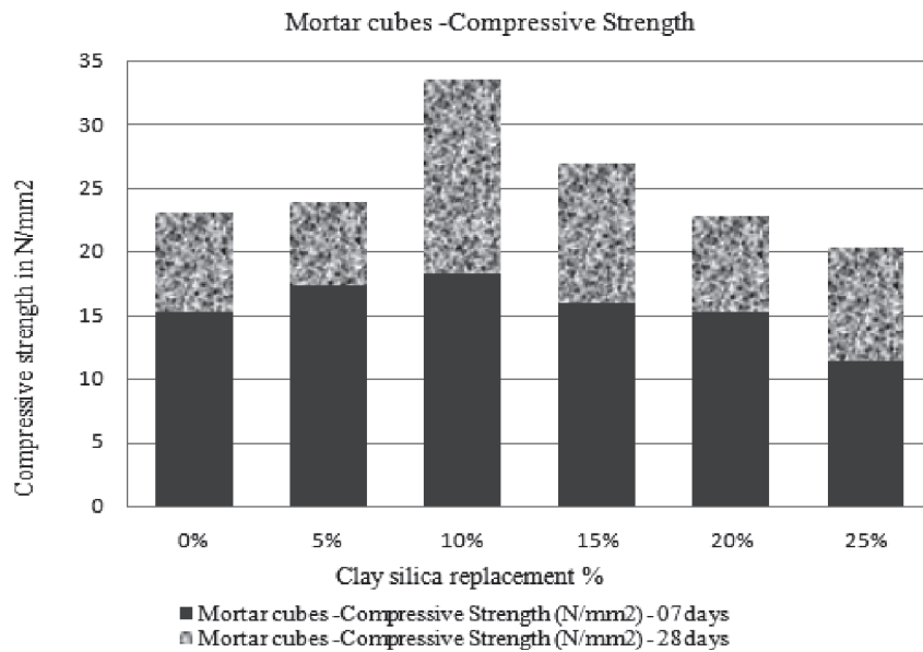
Fig. 2. Effect of clay silica in replacement of cement on the compressive strength of mortar cubes.
