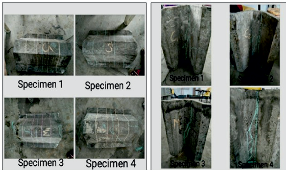
Fig. 6. Tested ferrocement panels with identified Crack pattern.
