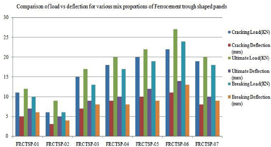
Fig. 5. Comparison of load vs deflection for various mix proportions of ferrocement trough shaped panels.
