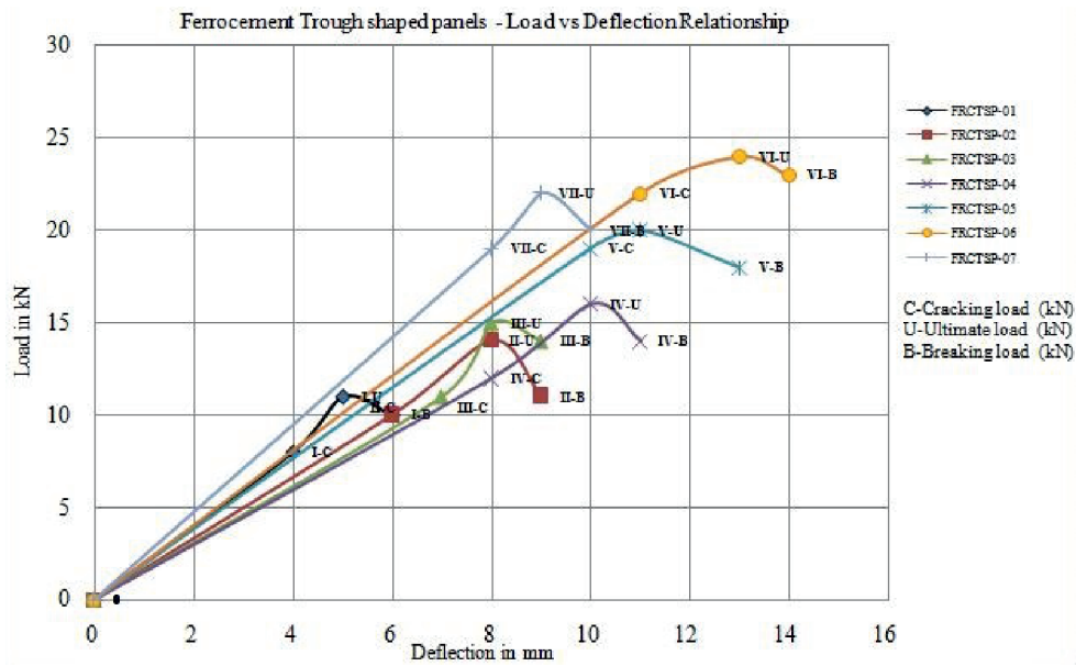
Fig. 4. Load capacity vs deflection of ferrocement panels.
