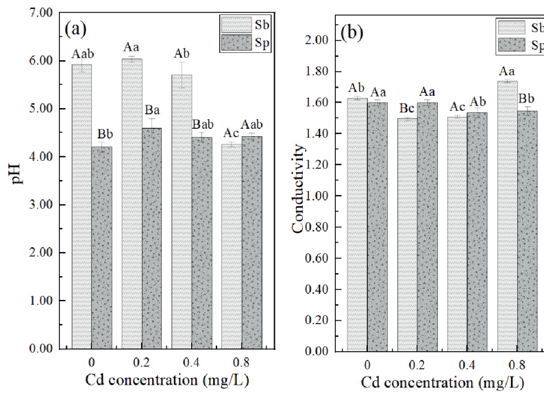
Fig. 4. Variations in pH a) and conductivity b) in the liquid culture medium of Sb and Sp. Note: Different lowercase letters indicate a significant difference between the same strain under different Cd concentrations ( P < 0.05 ), while different uppercase letters indicate a significant difference between the two strains under the same Cd concentration ( P < 0.05 ).
