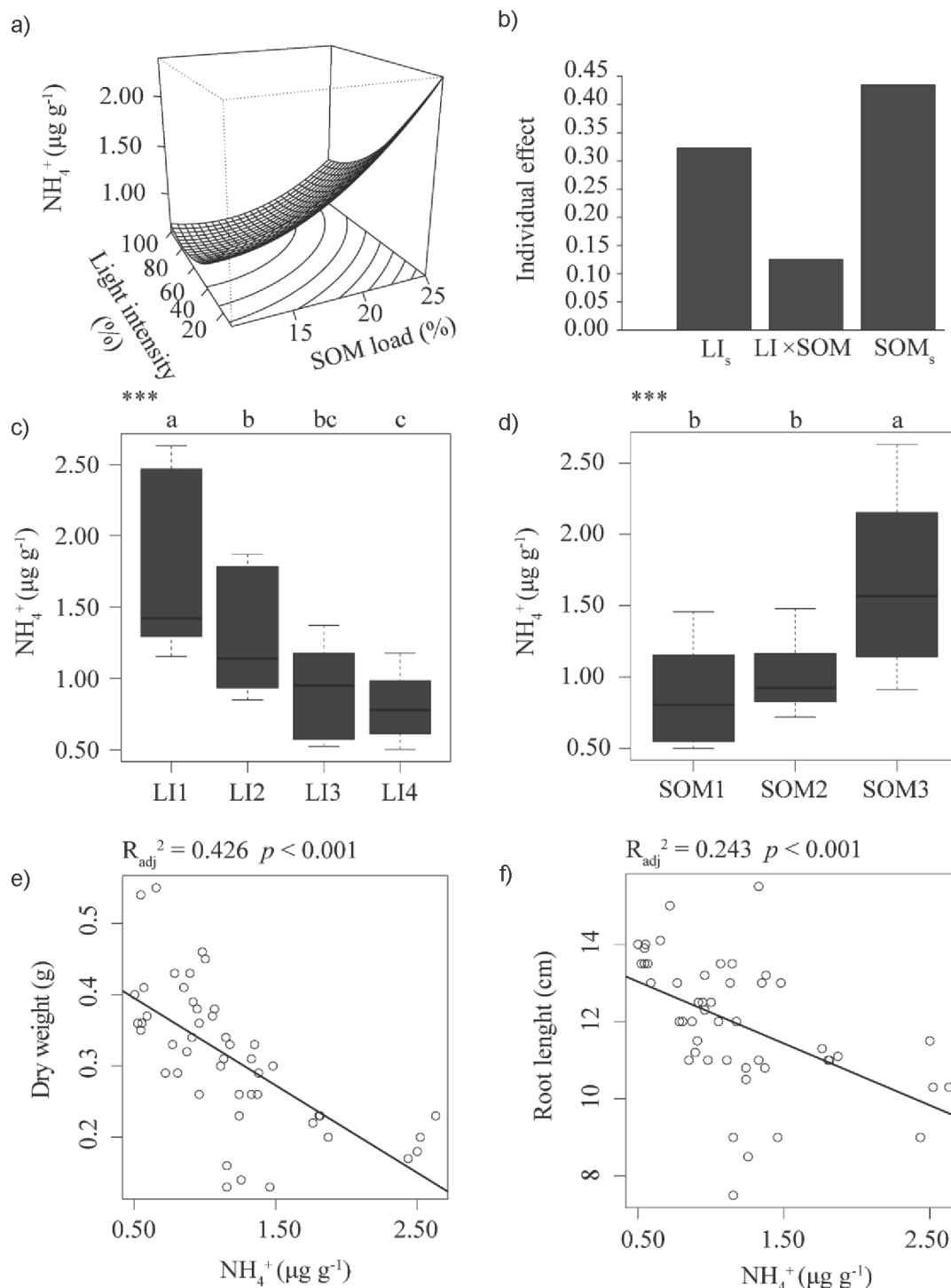
Fig. 2. Relationships between sediment \text{NH}_4^+ content and light intensity, SOM load, and growth characteristics of V. natans (n = 4). a. Effects of the interactions between light intensity and SOM on \text{NH}_4^+ content. b. Importance of each explanatory variable and group of variables on the variability in \text{NH}_4^+ content. c, d. \text{NH}_4^+ contents under various light intensity levels and SOM loads. e, f. Relationships between \text{NH}_4^+ content and the growth characteristics of V. natans . (LI: light intensity; \text{LI} \times \text{SOM} : interactions between light intensity and SOM load. LIs include LI and \text{LI}^2 ; SOMs include SOM and \text{SOM}^2 . LI1, LI2, LI3, and LI4 indicate 10%, 30%, 60%, and 100% natural light intensities, respectively. SOM1, SOM2, and SOM3 had initial SOM loads of 11%, 17%, and 25%, respectively.).
