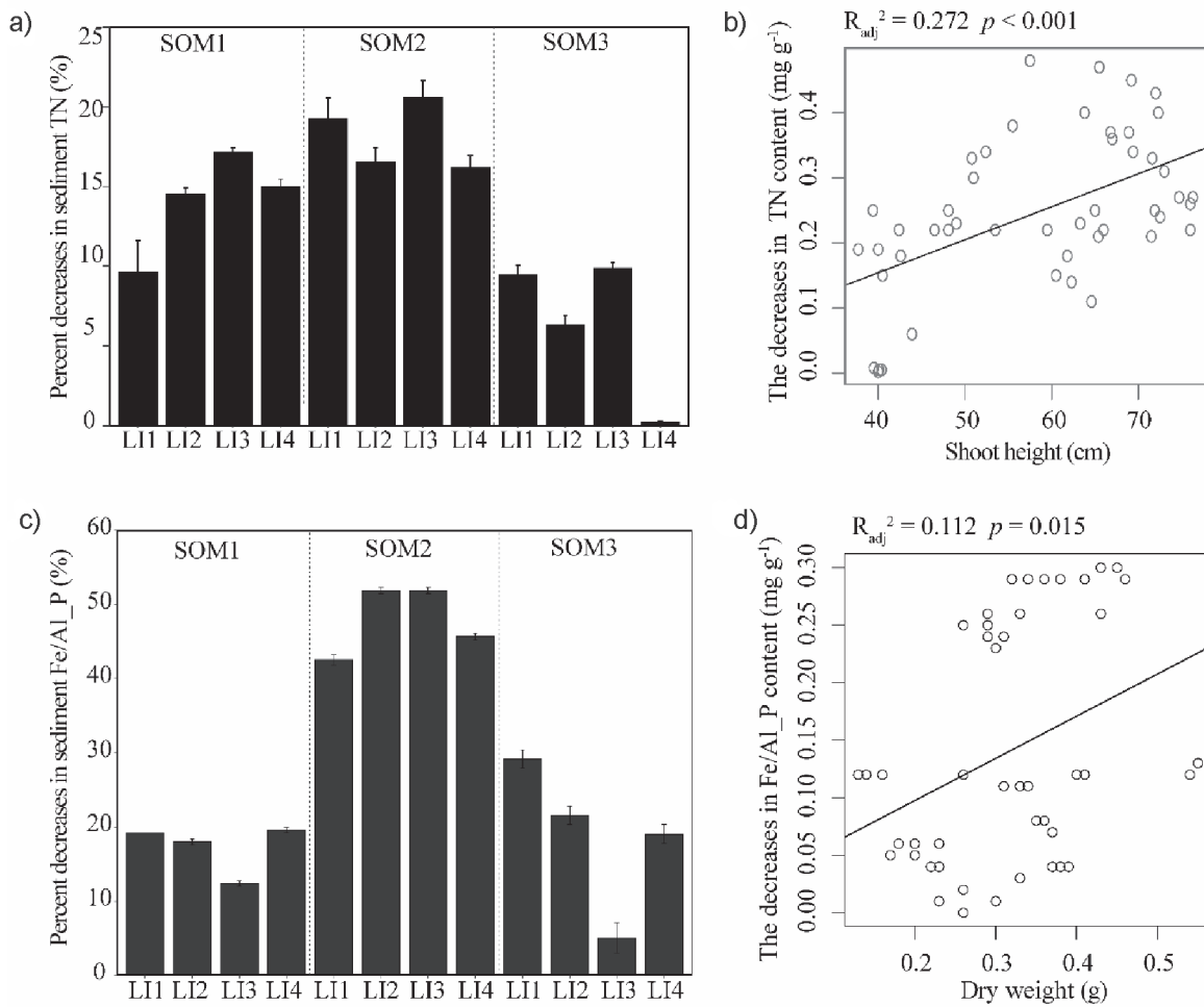
Fig. 4. Percent decreases in sediment total nitrogen (TN) and iron and aluminum phosphorus (Fe/Al-P) contents under different environmental conditions after 70 days and the relationships between TN and Fe/Al-P removal and the growth characteristics of V. natans (n = 4). (LI1, LI2, LI3, and LI4: 10%, 30%, 60%, and 100% natural light intensity, respectively. SOM1, SOM2, and SOM3 had initial SOM loads of 11%, 17%, and 25%, respectively.).
