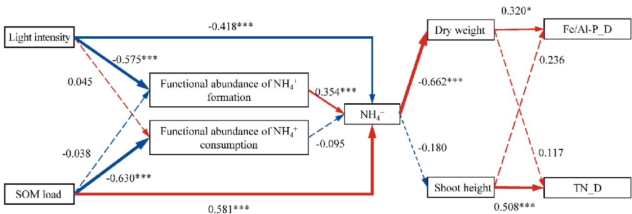
Fig. 5. Structural equation modeling representing the relationship between light intensity, SOM load, abundances of bacteria functional genes associated with NH 4 + formation and consumption, growth characteristics of V. natans , and decreases in sediment TN and Fe/Al-P contents. Solid lines indicate significant paths (n = 4; N = 48; * p<0.05; ** p<0.01; *** p<0.001). Dashed lines indicate non-significant paths (p>0.05). Red and blue colors indicate positive and negative path intensities, respectively. Numbers on the arrows are the normalized path coefficients, which indicate the strength of the influence of one factor on another. Arrow widths are proportional to the standard path coefficients denoted by the adjacent numbers.
