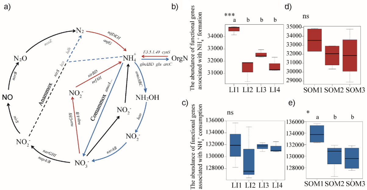
Fig. 3. Abundances of bacterial functional genes associated with \text{NH}_4^+ formation and consumption at different light intensity levels ( n = 3 ) and SOM loads ( n = 4 ). (LI1, LI2, LI3, and LI4: 10%, 30%, 60%, and 100% natural light intensity, respectively. SOM1, SOM2, and SOM3 had initial SOM loads of 11%, 17%, and 25%, respectively.).
