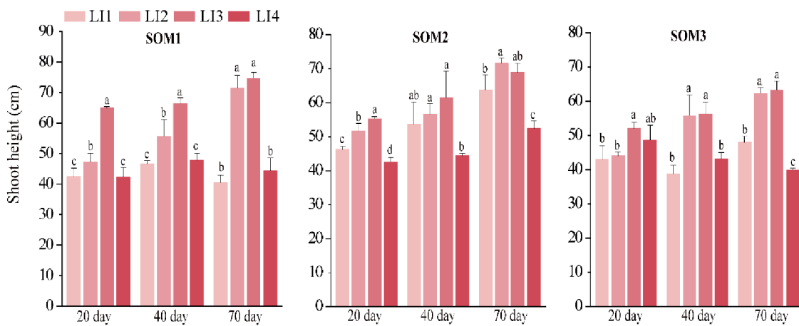
Fig. S3. The shoot height of V. natans after 20, 40 and 70 days (n = 4). (LI1, LI2, LI3, and LI4 indicate 10%, 30%, 60%, and 100% natural light intensity, respectively. SOM1, SOM2, and SOM3 had initial SOM loads of 11%, 17%, and 25%, respectively.)
