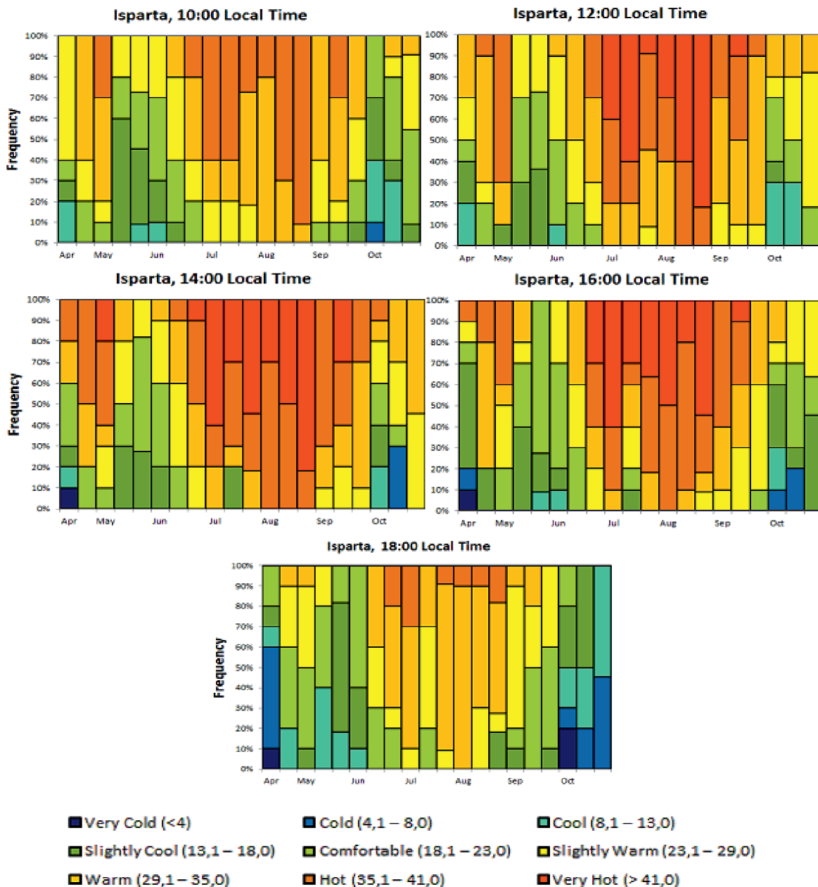
Fig. 4. Isparta city center PET distributions.
