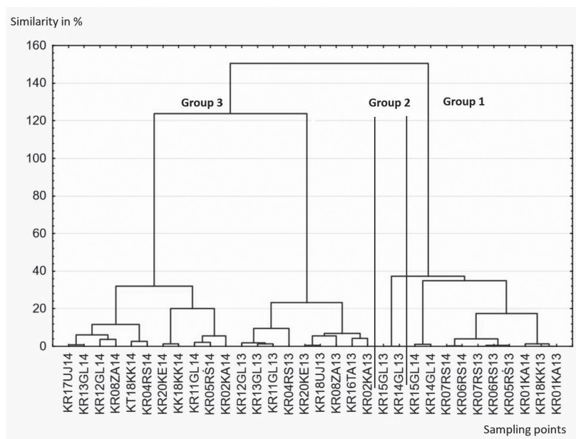
Fig. 2. Dendrogram of the cluster analysis according to Ward: the total content of heavy metals in the Kłodnica River sediments.
