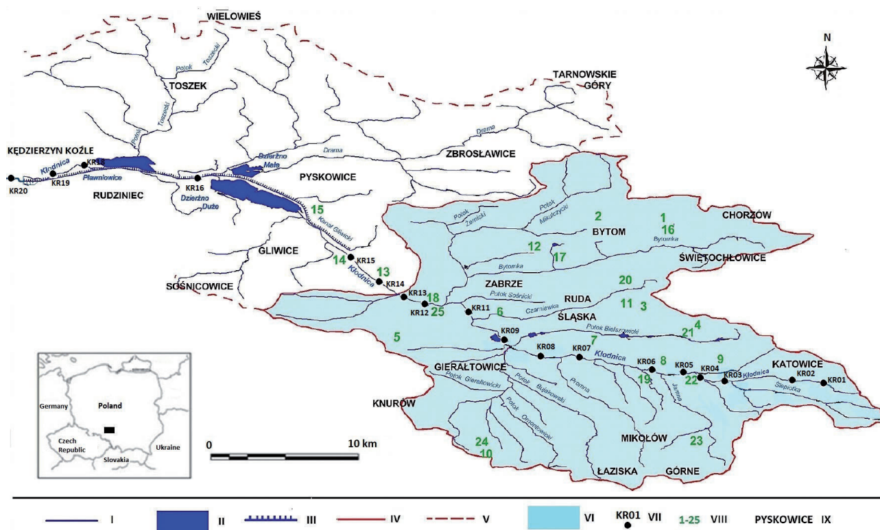
Fig. 1. Description of the area and sampling points on the Kłodnica River catchment: I – watercourses, II – reservoirs, III – canals, IV – the border of the Kłodnica catchment, V – the border of the Kłodnica catchment to Kłodnica profile, VI – the border of the Kłodnica catchment to Gliwice profile, VII – bottom sediment sampling points, VIII – localization of pollution points and wastewater treatment plants: (1-10) – coal-mining industry, (11-13) – smelters, (14, 15) – transport industry, (16-19) – the energy industry, (20) – chemical industry, (21-25) – wastewater treatment plants, IX – cities [based on 4].
