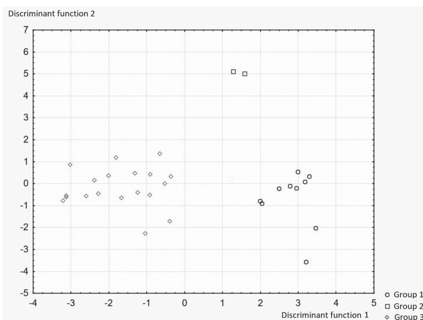
Fig. 3. Multivariate analysis of variance and discriminant analysis: the Kłodnica River sediments from years 2013-2014.
