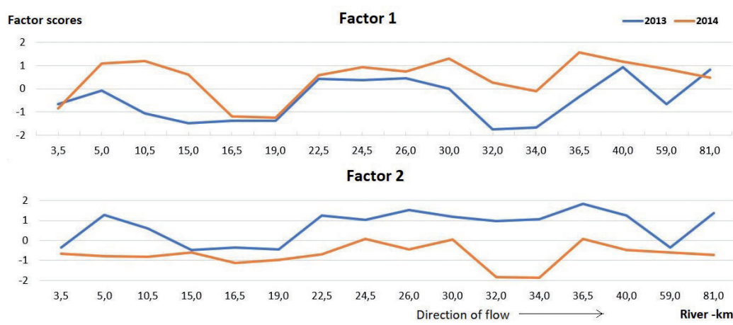
Fig. 4. Factor scores versus the distance of flow of the Kłodnica River.
