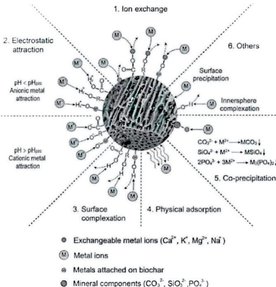
Fig. 2. Mechanisms of action of biochar on soil heavy metals.
