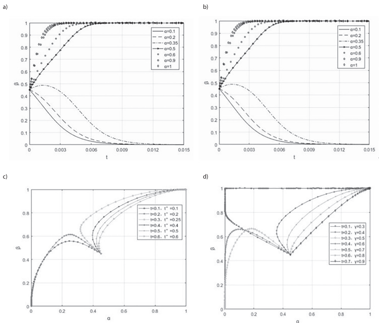
Fig. 1. Game evolution diagram.
