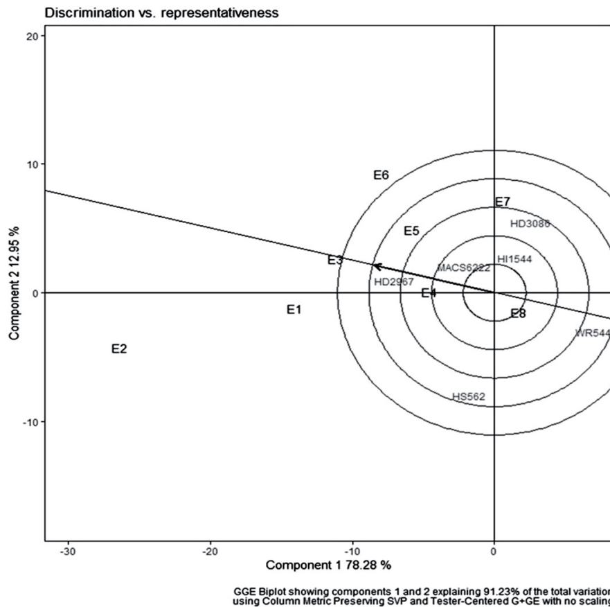
Fig. 2. Discrimination versus representativeness. Note: Four different dates of sowing: November 5 th (D1), November 25 th (D2), December 15 th (D3), and January 5 th (D4). These four different dates of sowing (D1, D2, D3, and D4) in the two years were treated to be a total of eight different environments (E1 to E8), considering the macro and micro environmental situations. So E1 was D1 in the first year of 2017-18, E2 was D2 in the first year of 2017-18, E3 was D3 in the first year of 2017-18, E4 was D4 in the first year of 2017-18, E5 was D1 in the second year 2018-19, E6 was D2 in the second year 2018-19, E7 was D3 in the second year 2018-19, and E8 was D4 in the second year 2018-19.
