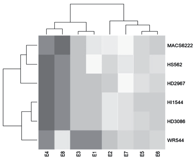
Fig. 1. Heat map for the performance of the different wheat genotypes for grain yield in the different environments. Note: Four different dates of sowing: November 5 th (D1), November 25 th (D2), December 15 th (D3), and January 5 th (D4). These four different dates of sowing (D1, D2, D3, and D4) in the two years were treated to be a total of eight different environments (E1 to E8), considering the macro and micro environmental situations. So E1 was D1 in the first year of 2017-18, E2 was D2 in the first year of 2017-18, E3 was D3 in the first year of 2017-18, E4 was D4 in the first year of 2017-18, E5 was D1 in the second year 2018-19, E6 was D2 in the second year 2018-19, E7 was D3 in the second year 2018-19, and E8 was D4 in the second year 2018-19.
