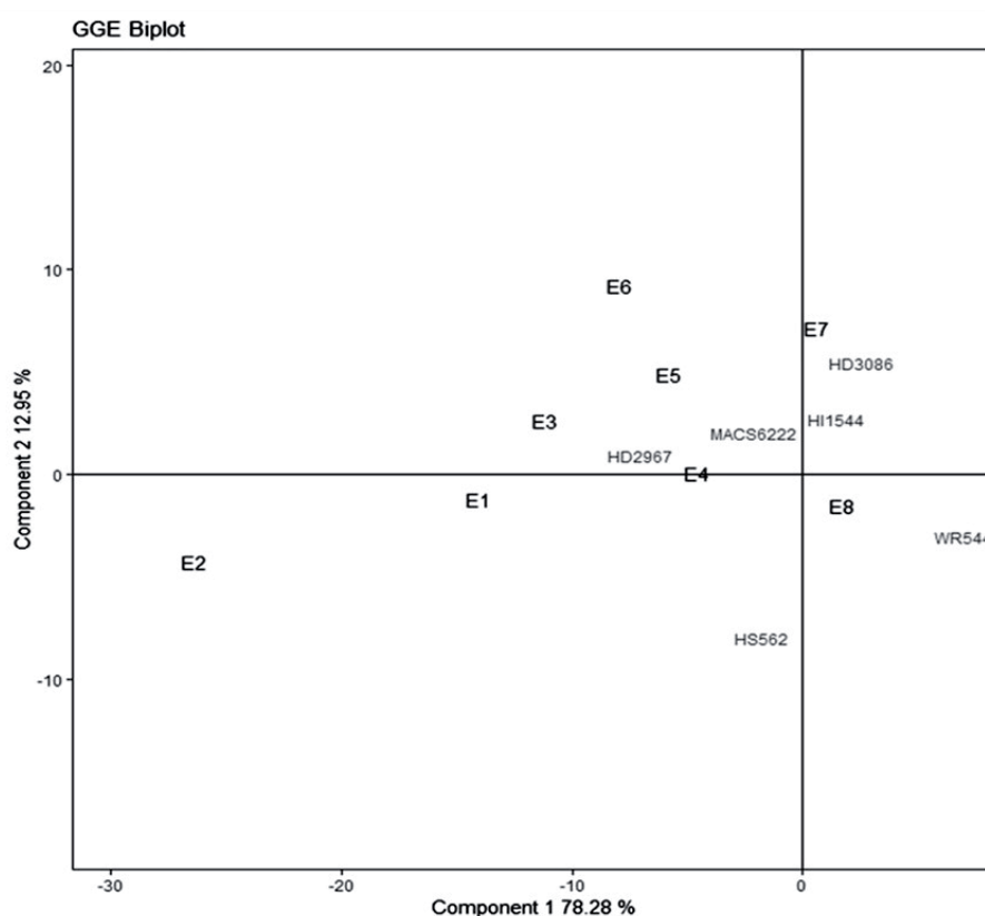
GGE Biplot showing components 1 and 2 explaining 91.23% of the total variation using Column Metric Preserving SVP and Tester-Centered G+GE with no scaling
