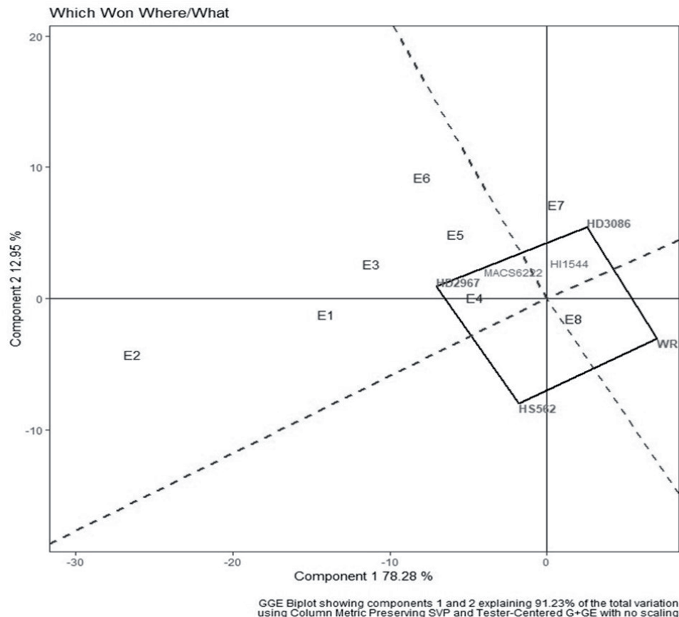
Fig. 5. Description of which won where what. Note: Four different dates of sowing: November 5 th (D1), November 25 th (D2), December 15 th (D3), and January 5 th (D4). These four different dates of sowing (D1, D2, D3, and D4) in the two years were treated to be a total of eight different environments (E1 to E8), considering the macro and micro environmental situations. So E1 was D1 in the first year of 2017-18, E2 was D2 in the first year of 2017-18, E3 was D3 in the first year of 2017-18, E4 was D4 in the first year of 2017-18, E5 was D1 in the second year 2018-19, E6 was D2 in the second year 2018-19, E7 was D3 in the second year 2018-19, and E8 was D4 in the second year 2018-19.
