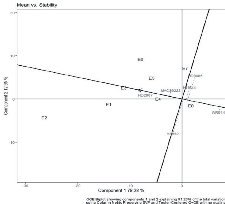
Fig. 4. GGE for Mean versus Stability. Note: Four different dates of sowing: November 5 th (D1), November 25 th (D2), December 15 th (D3), and January 5 th (D4). These four different dates of sowing (D1, D2, D3, and D4) in the two years were treated to be a total of eight different environments (E1 to E8), considering the macro and micro environmental situations. So E1 was D1 in the first year of 2017-18, E2 was D2 in the first year of 2017-18, E3 was D3 in the first year of 2017-18, E4 was D4 in the first year of 2017-18, E5 was D1 in the second year 2018-19, E6 was D2 in the second year 2018-19, E7 was D3 in the second year 2018-19, and E8 was D4 in the second year 2018-19.
