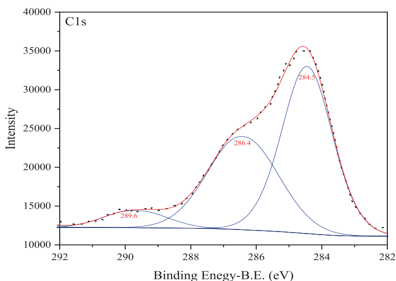
Fig. 7. The C1s spectra of Cd adsorbed palygorskite.
