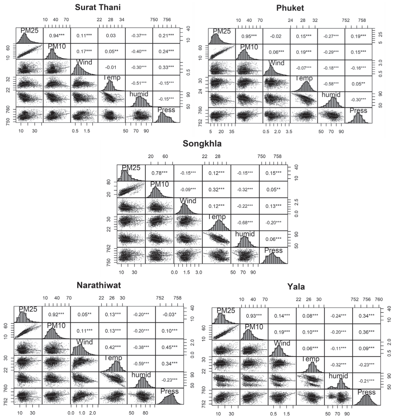
Fig. 4. Correlation between PM Concentration and Meteorological features from five stations in Southern Thailand.
