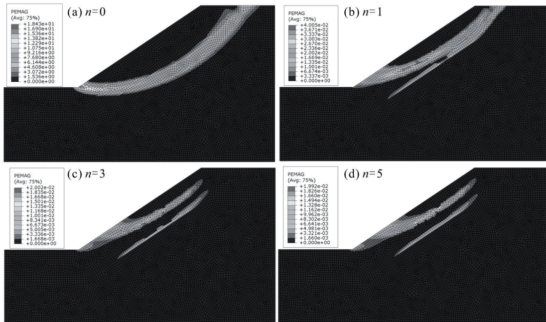
Fig. 7. The plastic strain distribution of expansive soil slopes under different numbers of dry-wet cycles.
