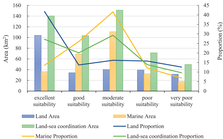
Fig. 6. Suitability classification.
