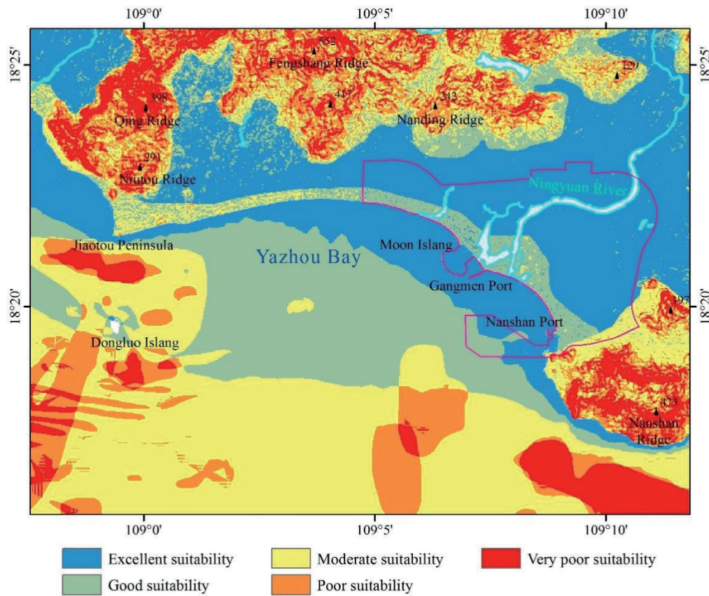
Fig. 5. Suitability zoning map for the construction of the Yazhou Bay project in Sanya based on land-sea coordination.
