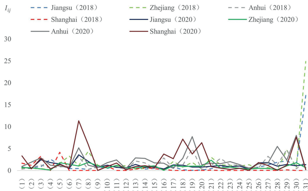
Fig. 12. The I_{ij} values evolution of the three provinces and municipality in the YRD in 2018 Vs. 2020.
