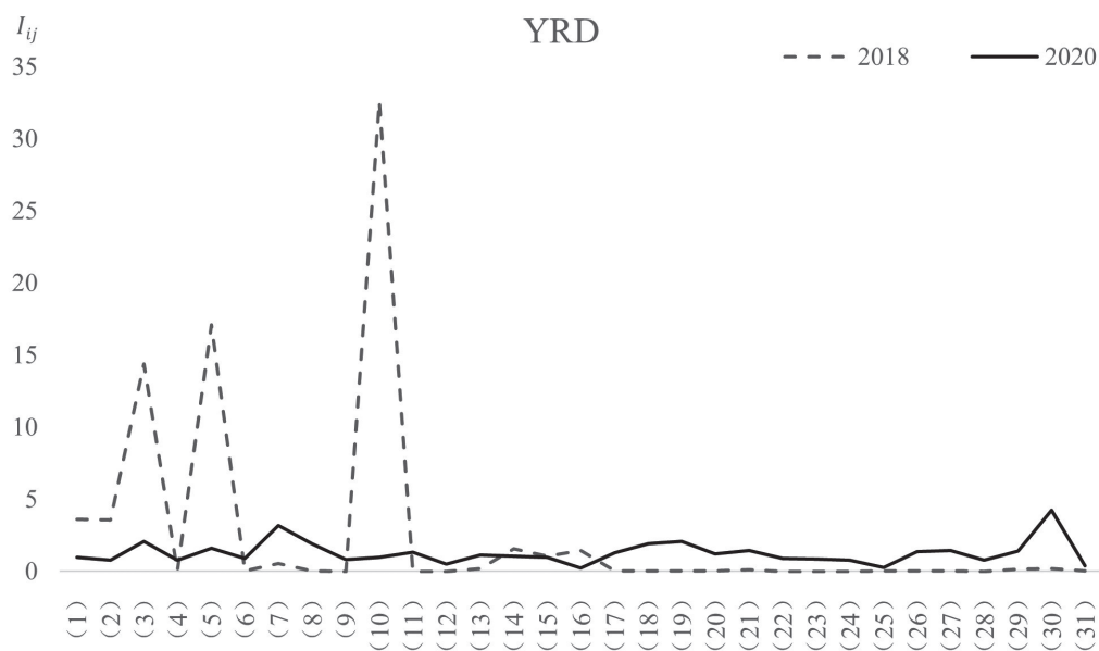
Fig. 7. The I_{ij} of MWPIIs in the YRD in 2018 Vs. 2020.
