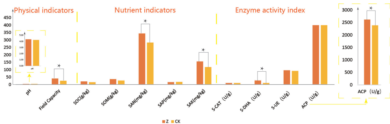
Fig. 1. Physicochemical and enzymatic indicators of soil under different planting modes. The asterisk topped the bars indicate significant differences (LSD test, P < 0.05 , n = 3 ).
