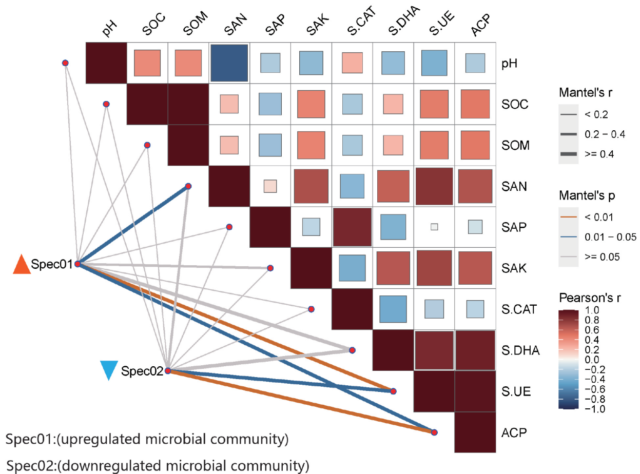
Fig. 5. Correlation analysis of environmental factors and their relationship with bacterial communities.
