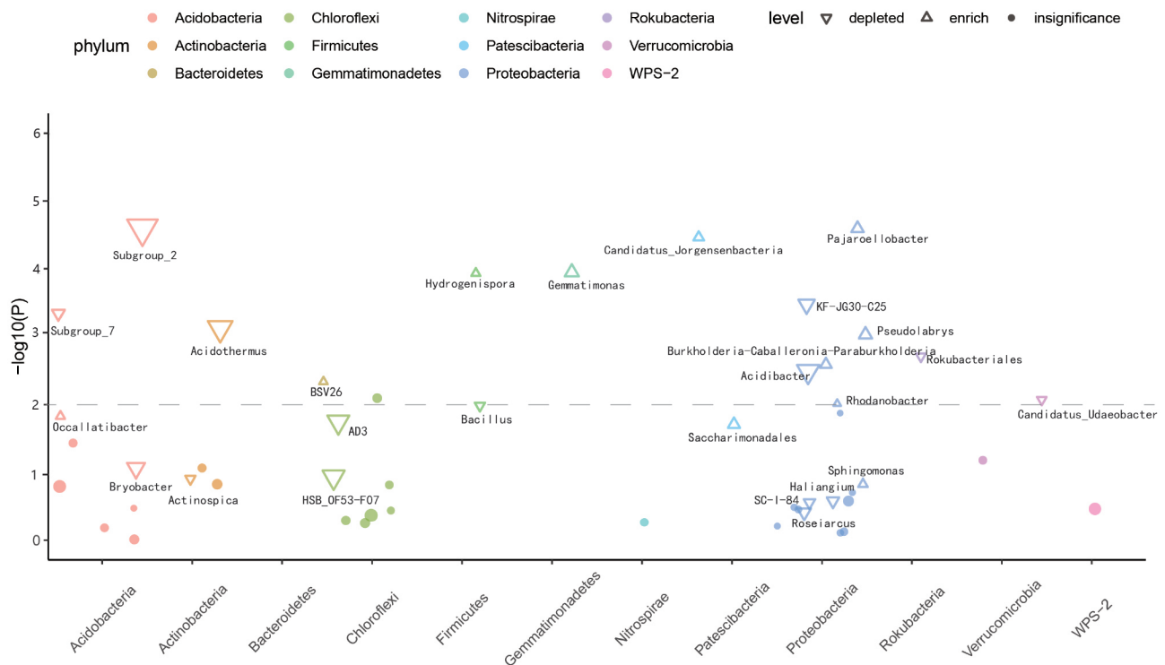
Fig. 4. Manhattan plot at the genus level. Each point on the plot represented a genus, with different genera categorized into different phyla. The size of the points reflected the magnitude of the fold change.
