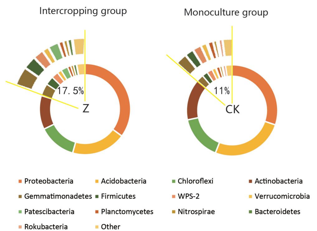
Fig. 3. Relative abundance of soil bacterial phyla in intercropping and monoculture systems.
