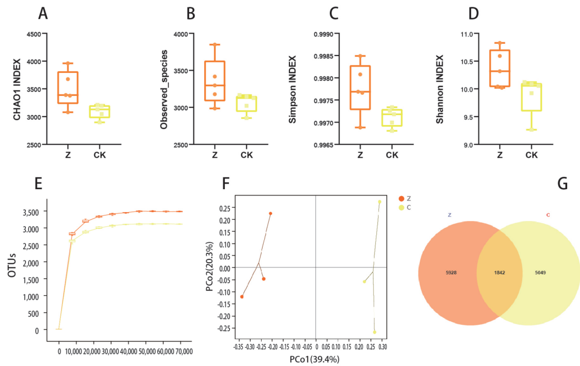
Fig. 2. (A) CHAO1 index, (B) Observed specifications index, (C) Simpson index, (D) Shannon index, (E) Rarefied fraction curves, (F) PCoA analysis of soil bacterial community, (G) Venn diagrams of core OTUs of soil bacteria in different planting modes.
