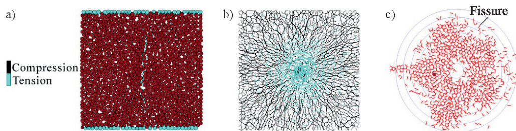
Fig. 11. Graphic illustration of grouting numerical calculation: a) Numerical simulation, b) Stress distribution c) Splitting form.
