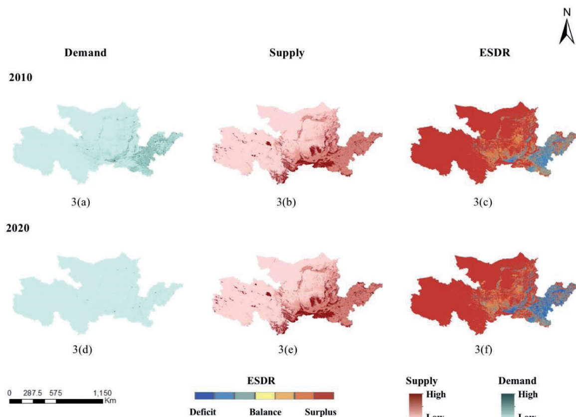
Fig. 3. Spatial Distribution of Supply and Demand of Carbon Sequestration Services.
