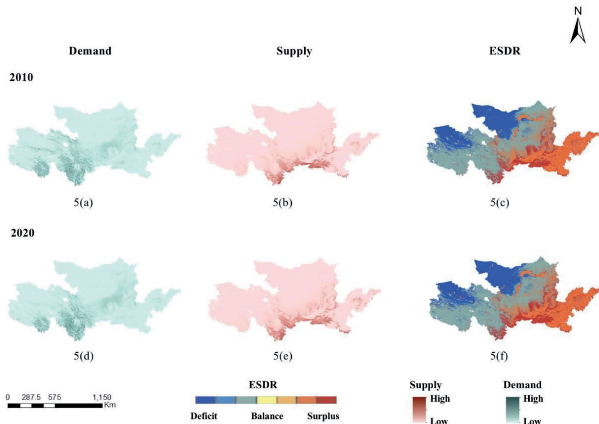
Fig. 5. Spatial Distribution of Supply and Demand of Soil Conservation Services.
