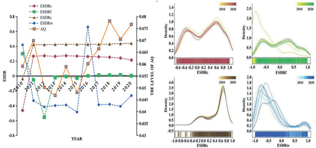
Fig. 7. Time Series Evolution and Kernel Density Analysis of the ESDR.
