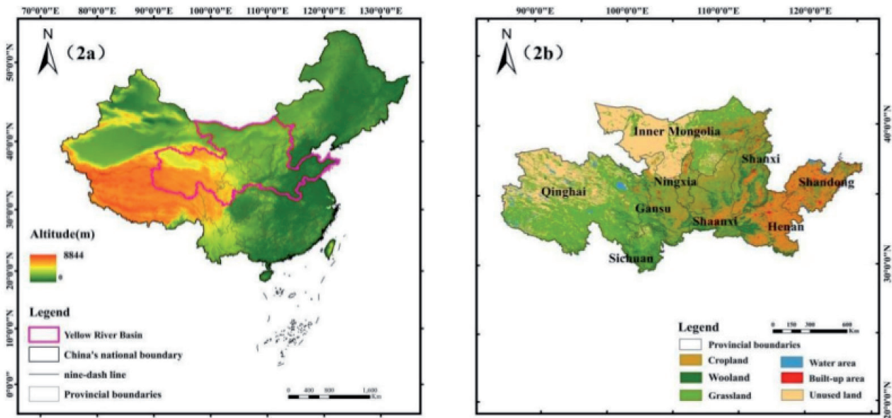
Fig. 2. Geographical Location and Land Use Situation of the Study Area.
