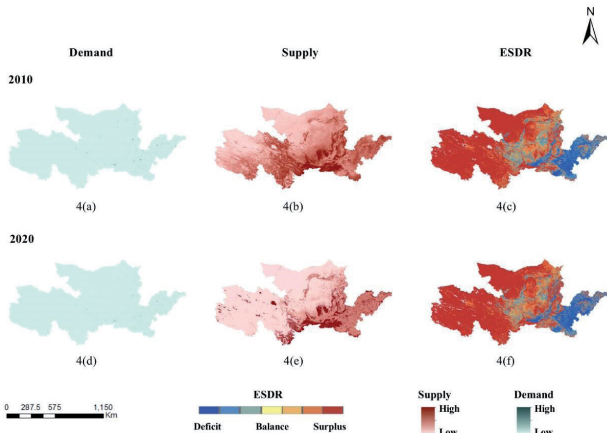
Fig. 4. Spatial Distribution of Supply and Demand of Food Production Services.
