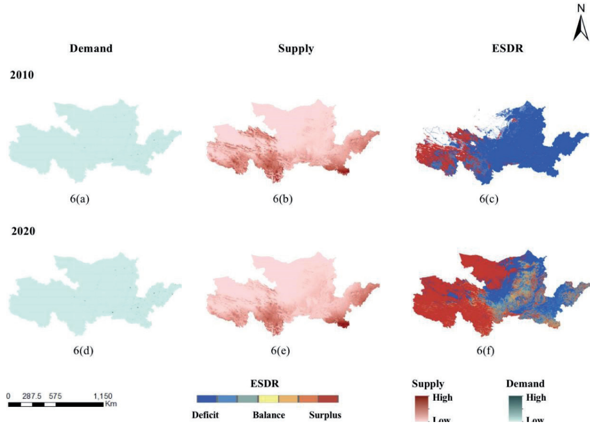
Fig. 6. Spatial Distribution of Supply and Demand of Water Conservation Services.
