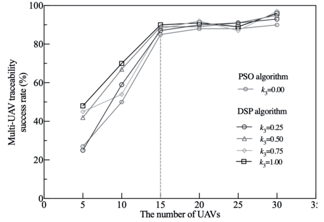
Fig. 6. The relationship between the number of UAVs and the success rate of traceability.
