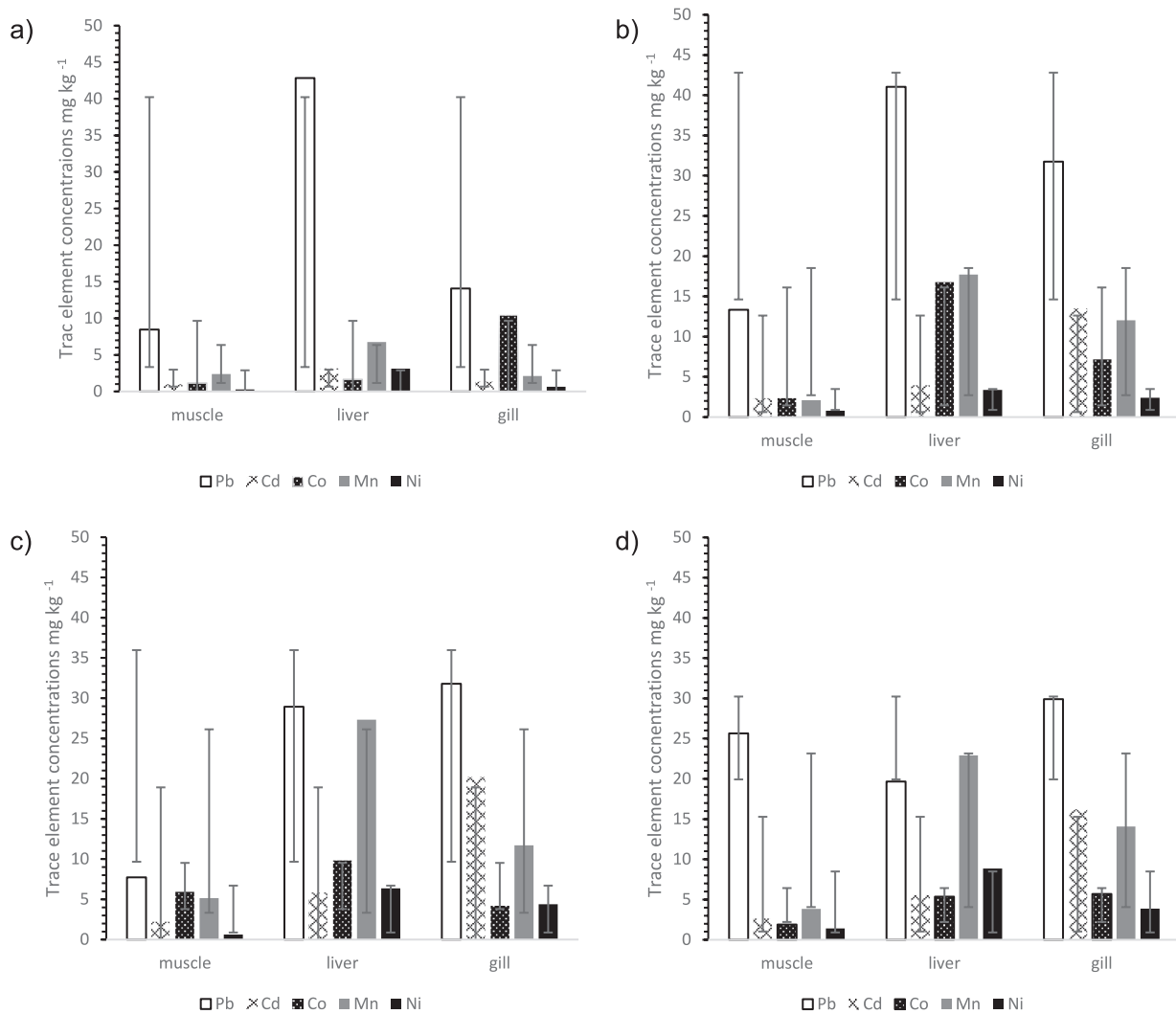
Fig. 3. Spatial variation of trace element levels in Aspius vorax fish species tissues caught in Tigris River of Baghdad City during March 2022 to February 2023 : site 1a), site 2 b), site 3 c) and site 4 d).
