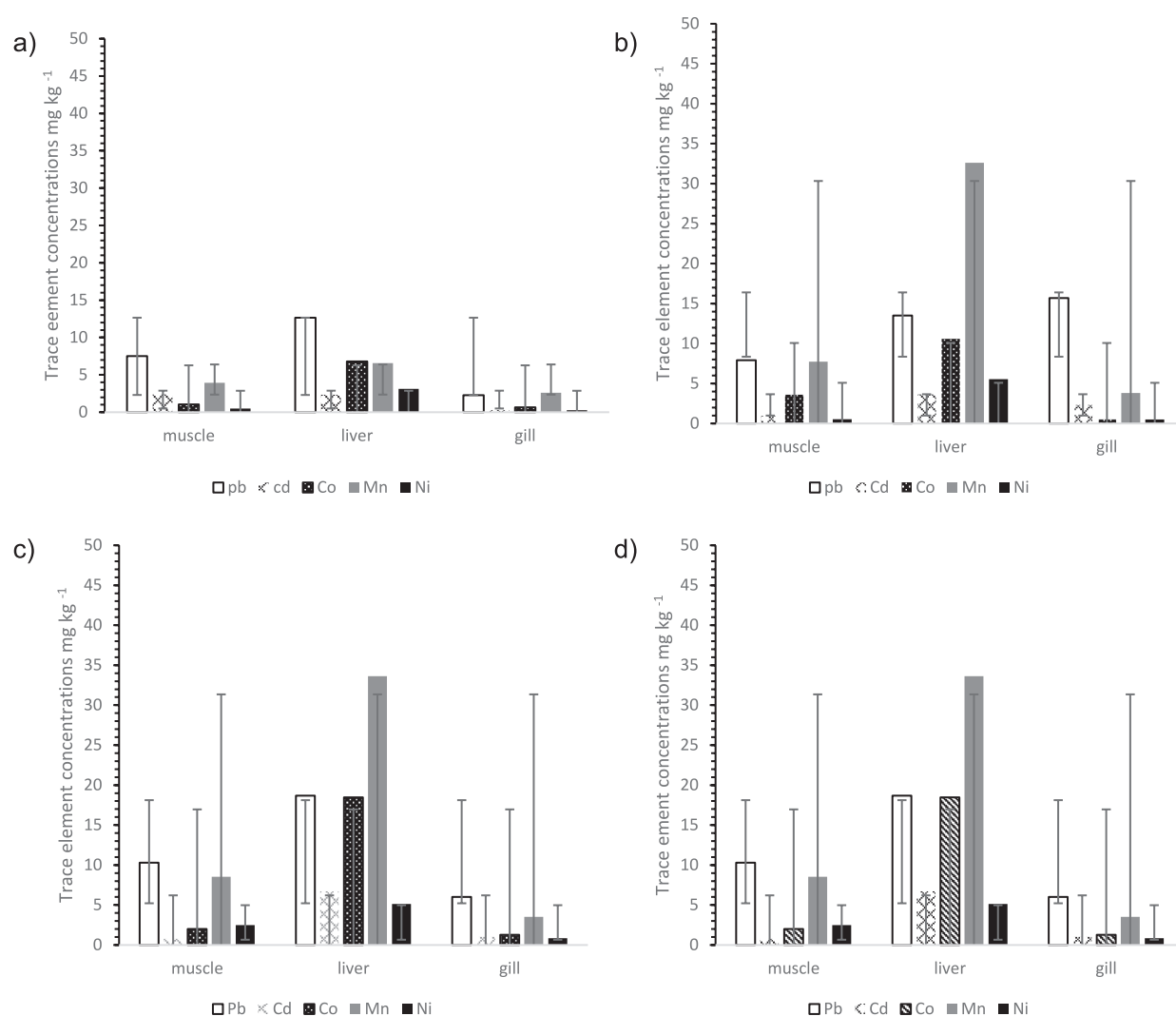
Fig. 2. Spatial variation of trace element levels in Cyprinus carpio fish species tissues caught in Tigris River of Baghdad City during March 2022 to February 2023: site 1 a), site 2 b), site 3 c) and site 4 d).
