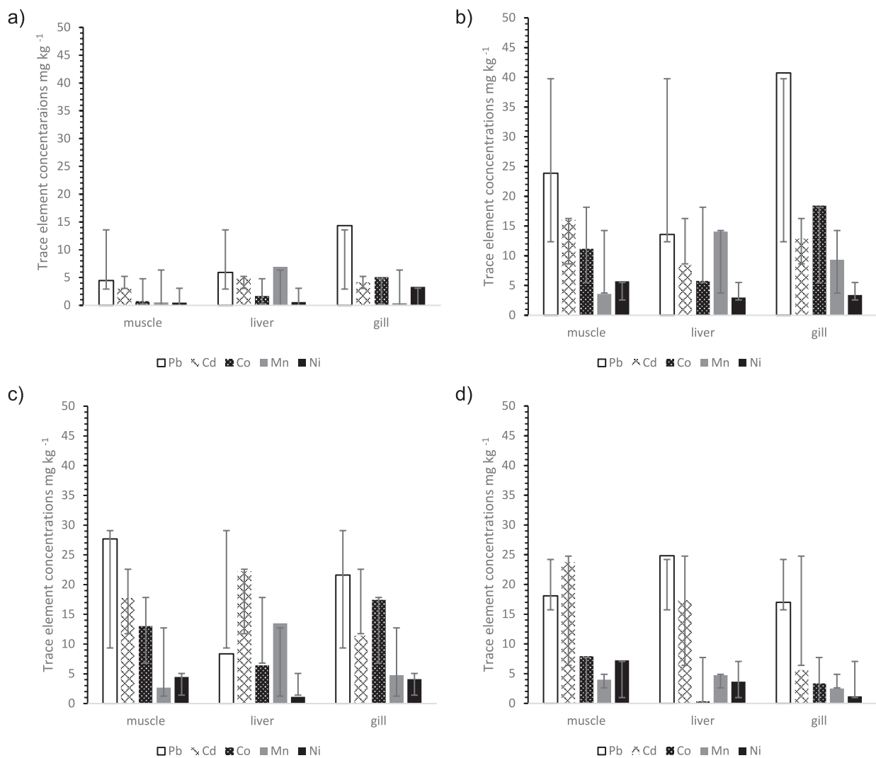
Fig. 4. Spatial variation of trace element levels Barbus xanthopterus fish species tissues caught in Tigris River of Baghdad City during March 2022 to February 2023: site 1 a), site 2 b), site 3 c) and site 4 d).
