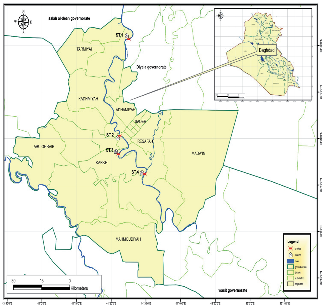
Fig. 1. Location of the studied sites in the Tigris River within Baghdad City Rashdea Area (site 1), Bab Al-Muazam Area (site 2), Al- Doura Area (Site 3), Al- Zafaraniya area (site 4) sampled during March 2022 to February 2023.
