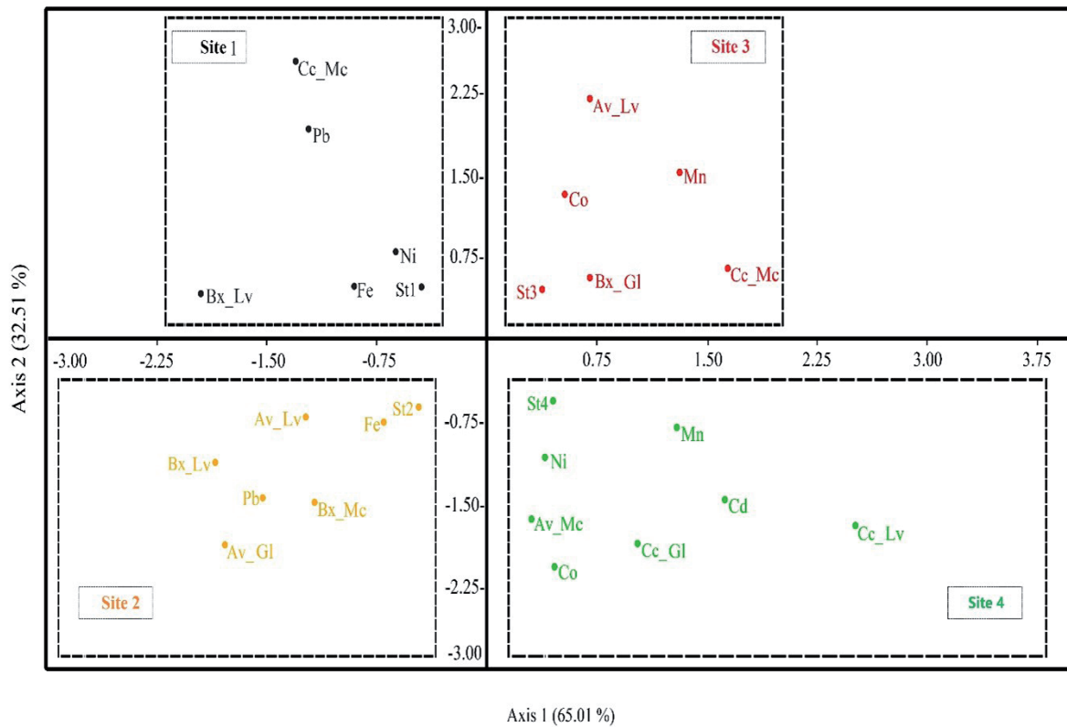
Fig. 5. Canonical correspondence analysis on mean values of several trace elements Fe (Iron), Pb (Lead), Cd (Cadmium), Co (Cobalt), Mn (Manganese) and Ni (Nickel) for three fish species Cc ( Cyprinus carpio ), Av ( Aspius vorax ), Bx ( Barbus xanthopterus ) in different fish tissues Mc (muscle), Lv (liver) and Gl (gill). Four sampled sites in the Tigris river within Baghdad City during March 2022 to February 2023 St1 (site 1), St2 (site 2), St3 (site 3) and St4 (site 4).
