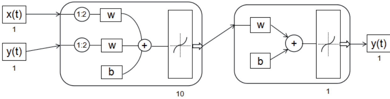
Fig. 2. NARX neural network structure diagram.
