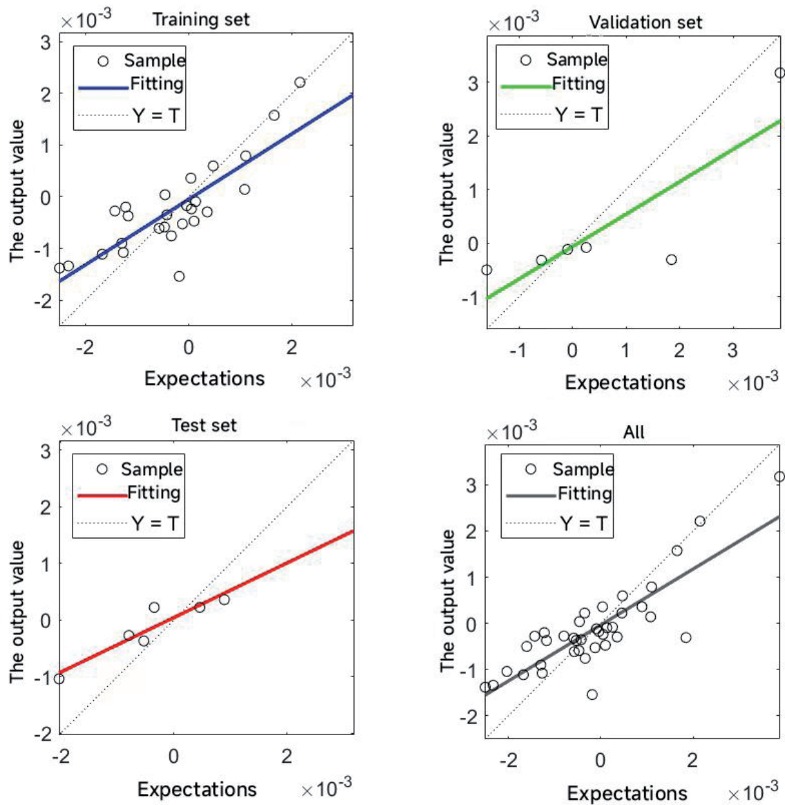
Fig. 9. NARX neural network regression effect diagram.
