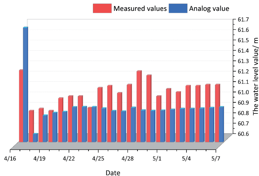
Fig. 5. Calibration results of one-dimensional hydrodynamic model.
