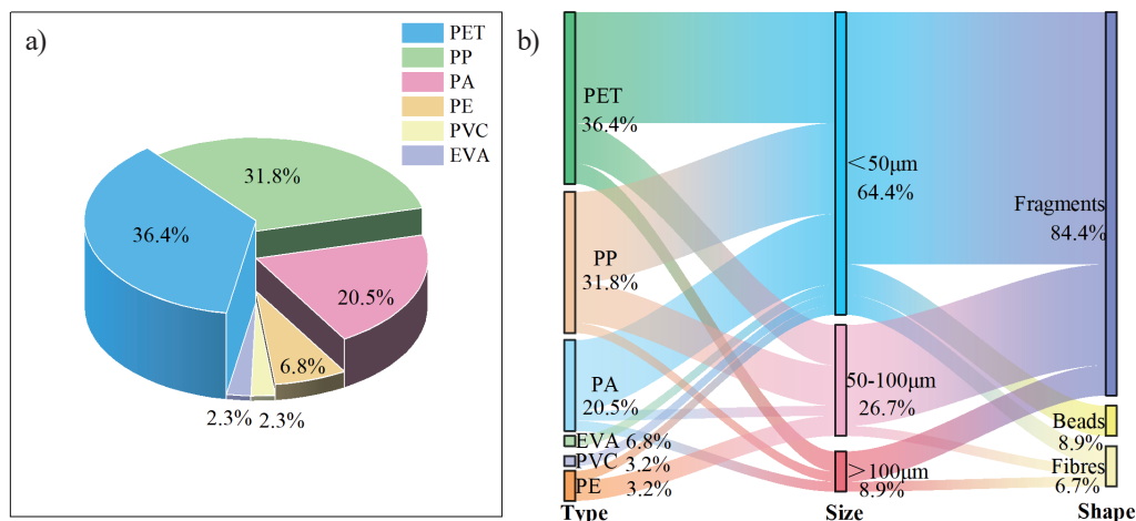
Fig. 5. a) Abundance of microplastic types in the surface water across all sites; b) characteristics of surface water microplastics.
