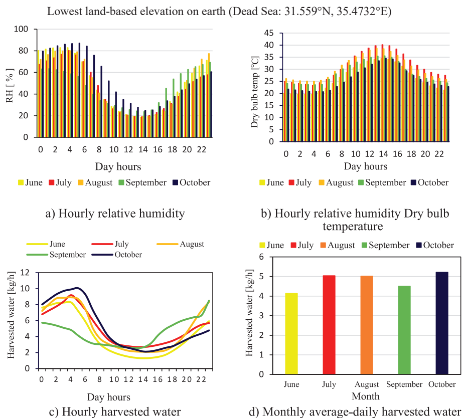
Fig. 10. Variation of RH, dry bulb temperature, amount of harvested water with time at average days of June- October 2023 at the lowest land-based elevation on earth (Dead Sea: 31.559°N, 35.4732°E).
