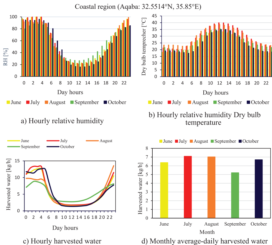
Fig. 8. Variation of RH, dry bulb temperature, and amount of harvested water with the time at average days of June- October 2023 at coastal region (Aqaba).
