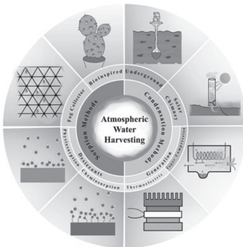
Fig. 1. Techniques for atmospheric water extraction [32].
