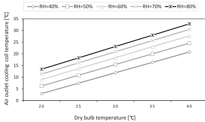
Fig. 7. Variation of design air outlet from evaporator with dry bulb temperature for different relative humidities.
