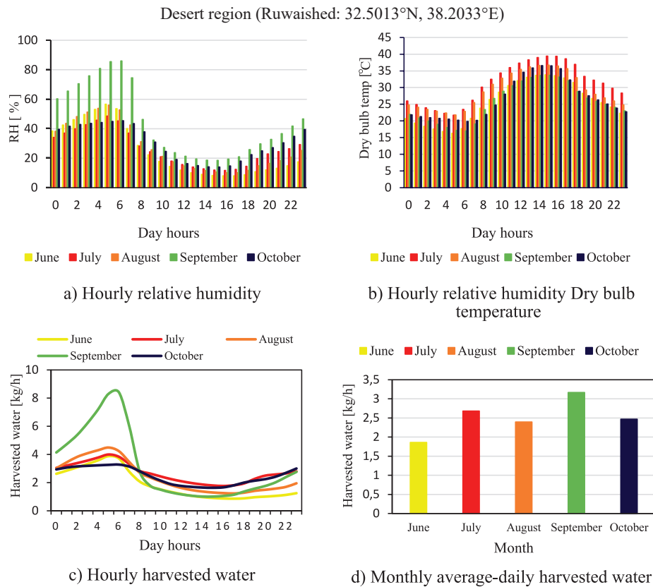
Fig. 11. Variation of RH, dry bulb temperature, and amount of harvested water with time at average days of June- October 2023 at a desert region (Ruwaished: 32.5013°N, 38.2033°E).
