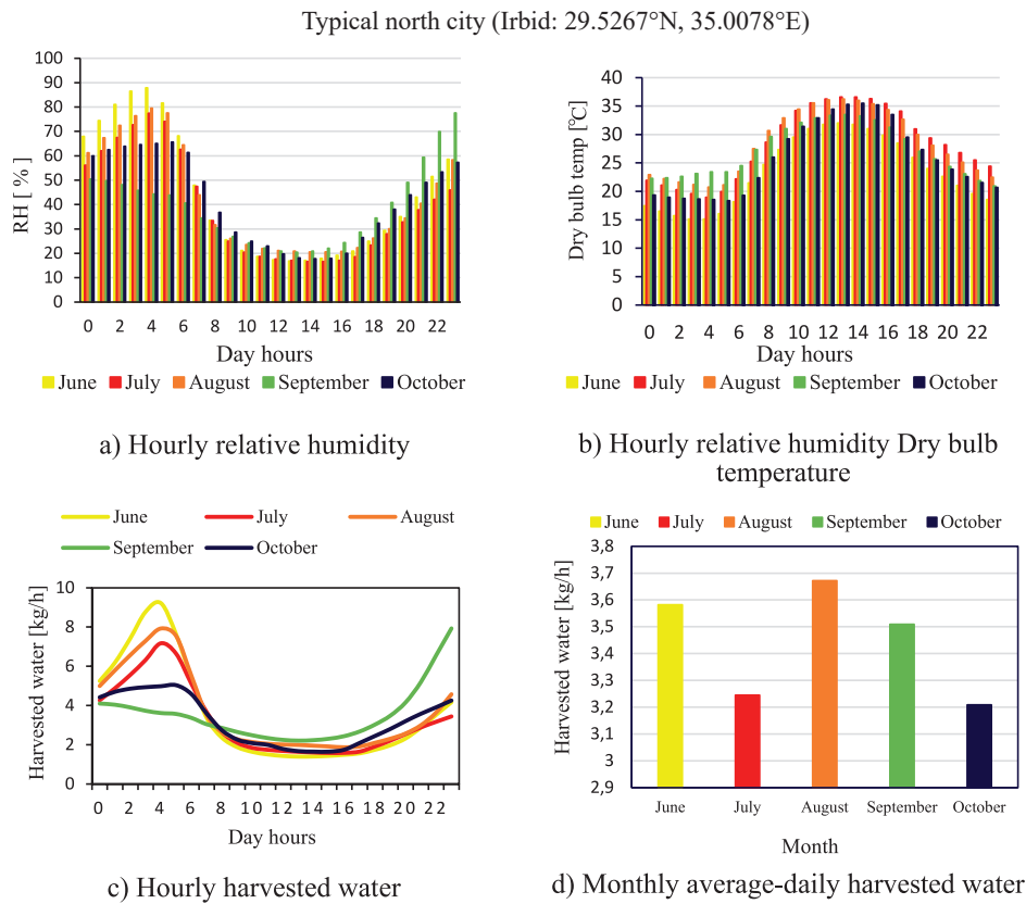
Fig. 9. Variation of RH, dry bulb temperature, and amount of harvested water with time at average days of June- October 2023 at a typical north city (Irbid: 29.5267°N, 35.0078°E).
