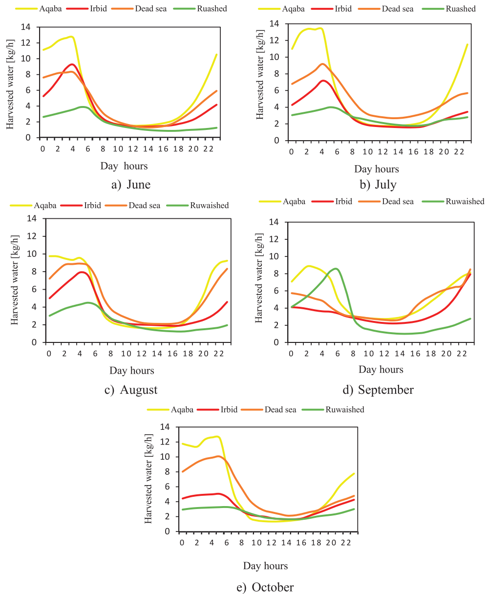
Fig. 12. Amount of harvested water with time at average days of June- October 2023 for different regions.
