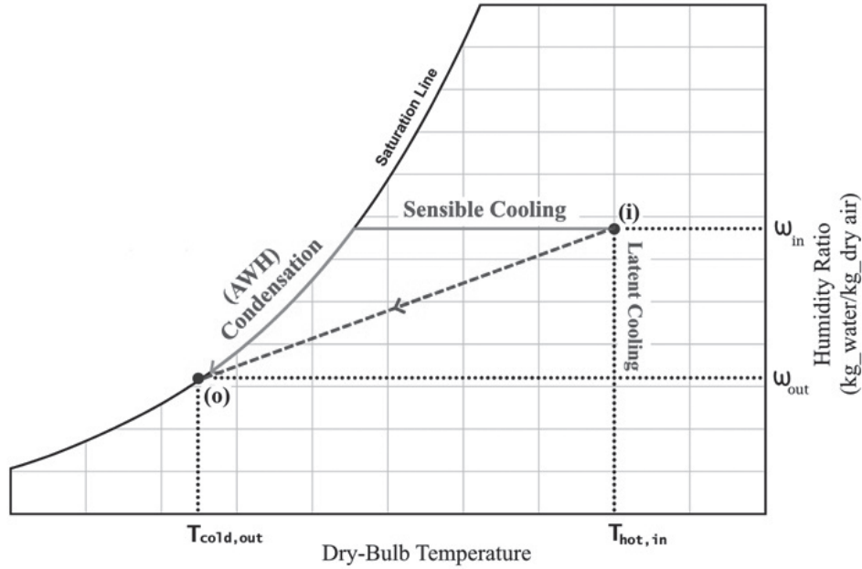
Fig. 4. AWH-Dehumidification process through evaporator by cooling the air below the dew point temperature, causing condensation.
