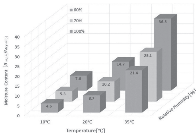
Fig. 3. The correlation among relative humidity, temperature, and atmospheric moisture content [36].
