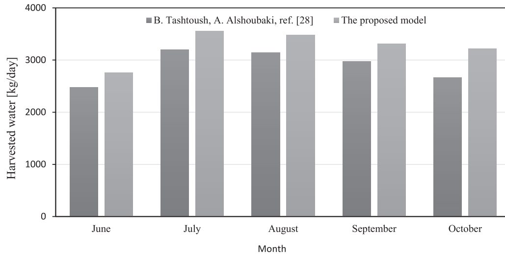
Fig. 14. Comparison of total daily atmospheric water collected for the studied regions during June- October 2023 as compared to (B. Tashtoush, A. Alshoubaki, ref. [28]).
