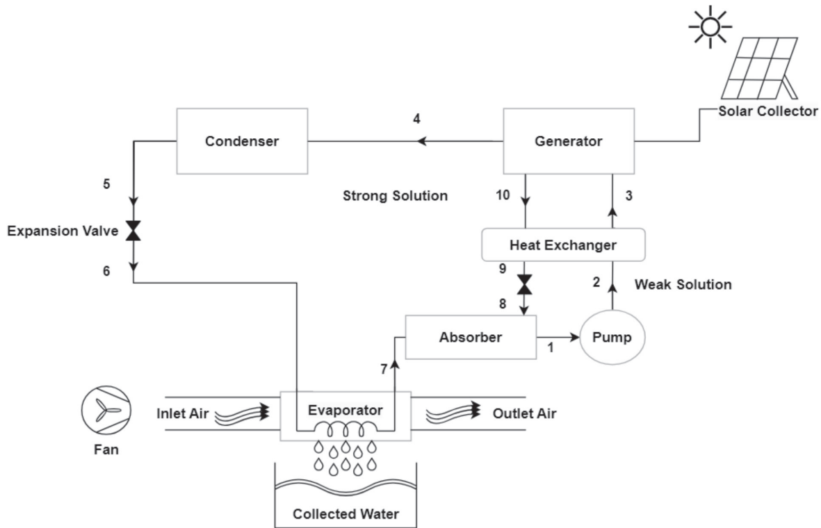
Fig. 2. Schematic diagram of solar absorption cool cycle augmented atmospheric water harvesting system.
