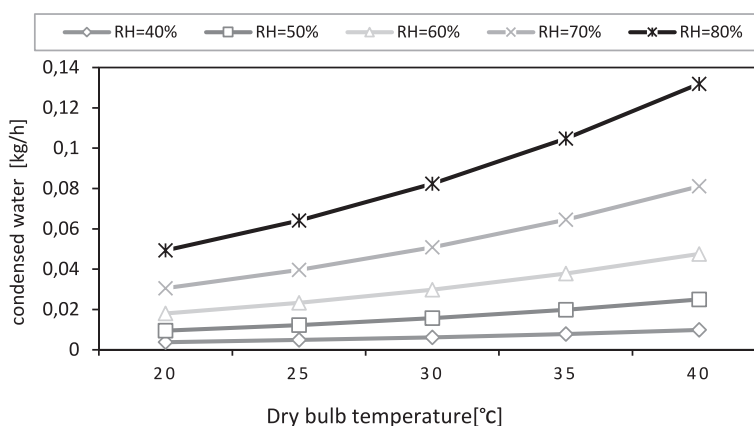
Fig. 6. Variation of water condensation rate with dry bulb temperature for different relative humidities for 5 kW evaporator cooling capacity.
