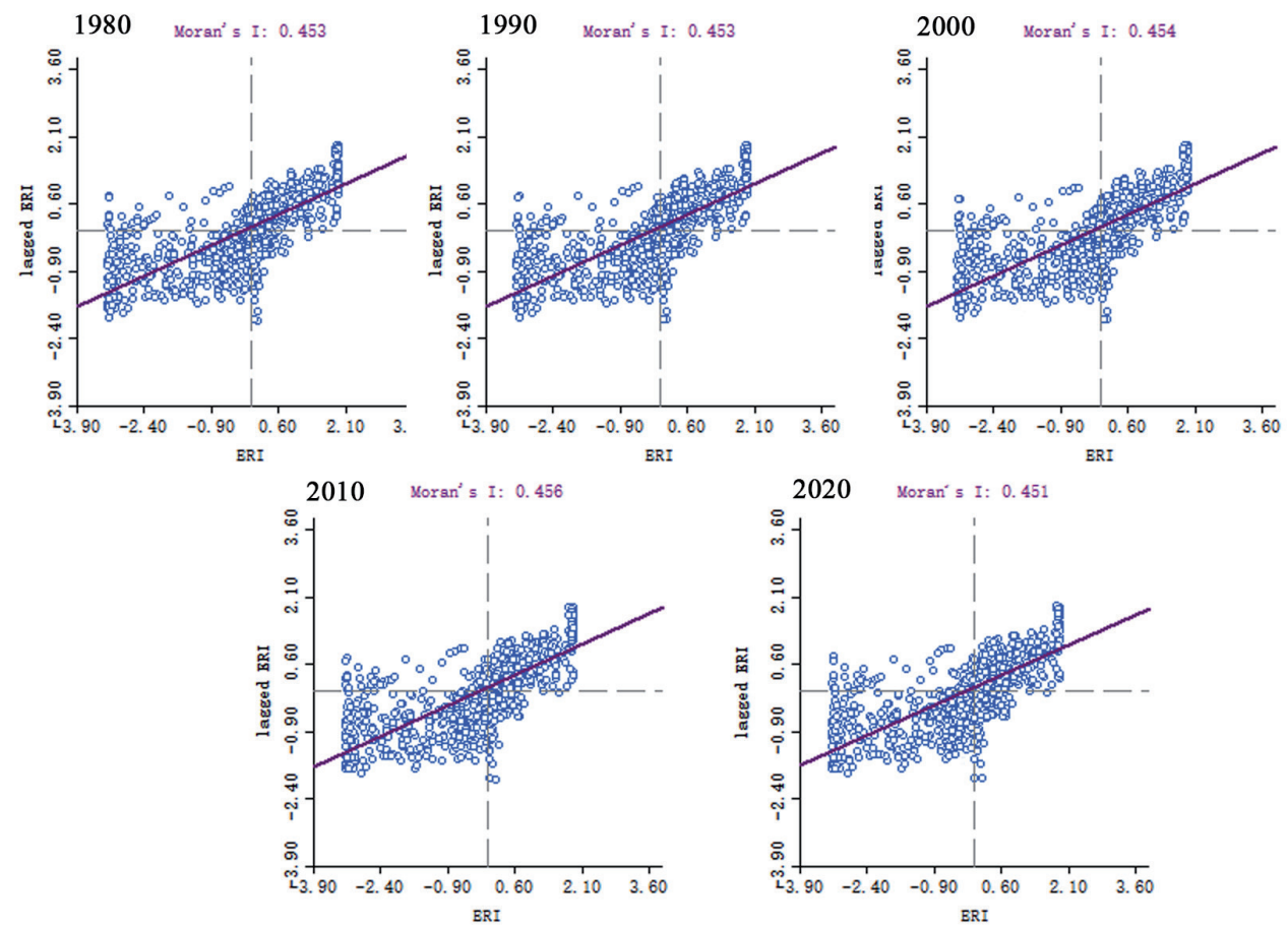
Fig. 7. Global spatial autocorrelation of ecological risk in Hainan from 1980 to 2020.
