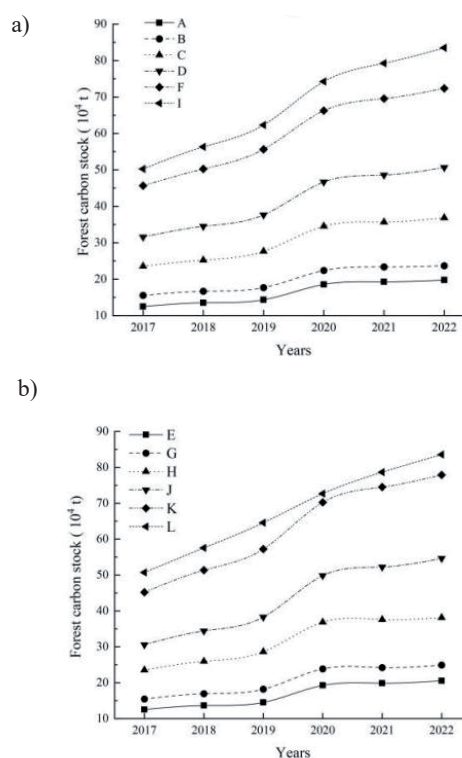
Fig. 3. Changes in forest carbon storage in survey sites from 2017 to 2022. a) Forest carbon storage in the control group, b) Forest carbon storage in the experimental group.
