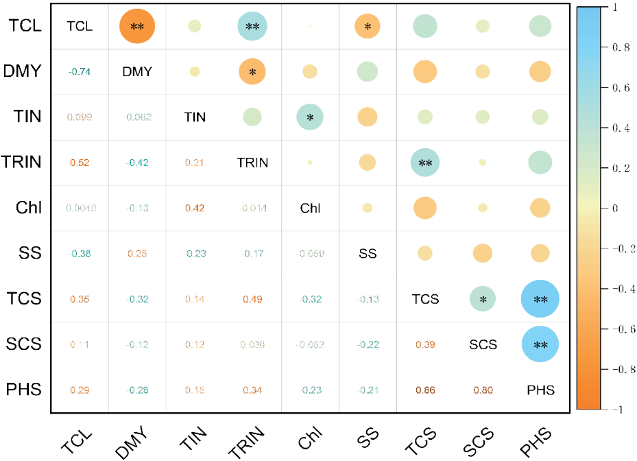
Fig. 4. Correlation analysis between efficacy components, calcium content, and physiological and biochemical indexes of N. grossedentata . The correlation between nine physiological indicators is shown in the figure; the horizontal and vertical coordinates are nine different physiological indicators. Values in the table are the Pearson correlation coefficient. Close to 1 indicates a stronger positive correlation, close to -1 indicates a stronger negative correlation and close to 0 indicates no correlation. * P \leq 0.05 ; ** P \leq 0.01 indicates extremely significant. TCL-Total calcium content of leaves; DMY-Dihydrosalicylate; TIN-Myricetin; TRIN-Myricetin; Chl-Chlorophyll; SS-Soluble sugar; TCS-Total calcium of soil; SCS-Soluble calcium of soil; PHS-PH of soil.
