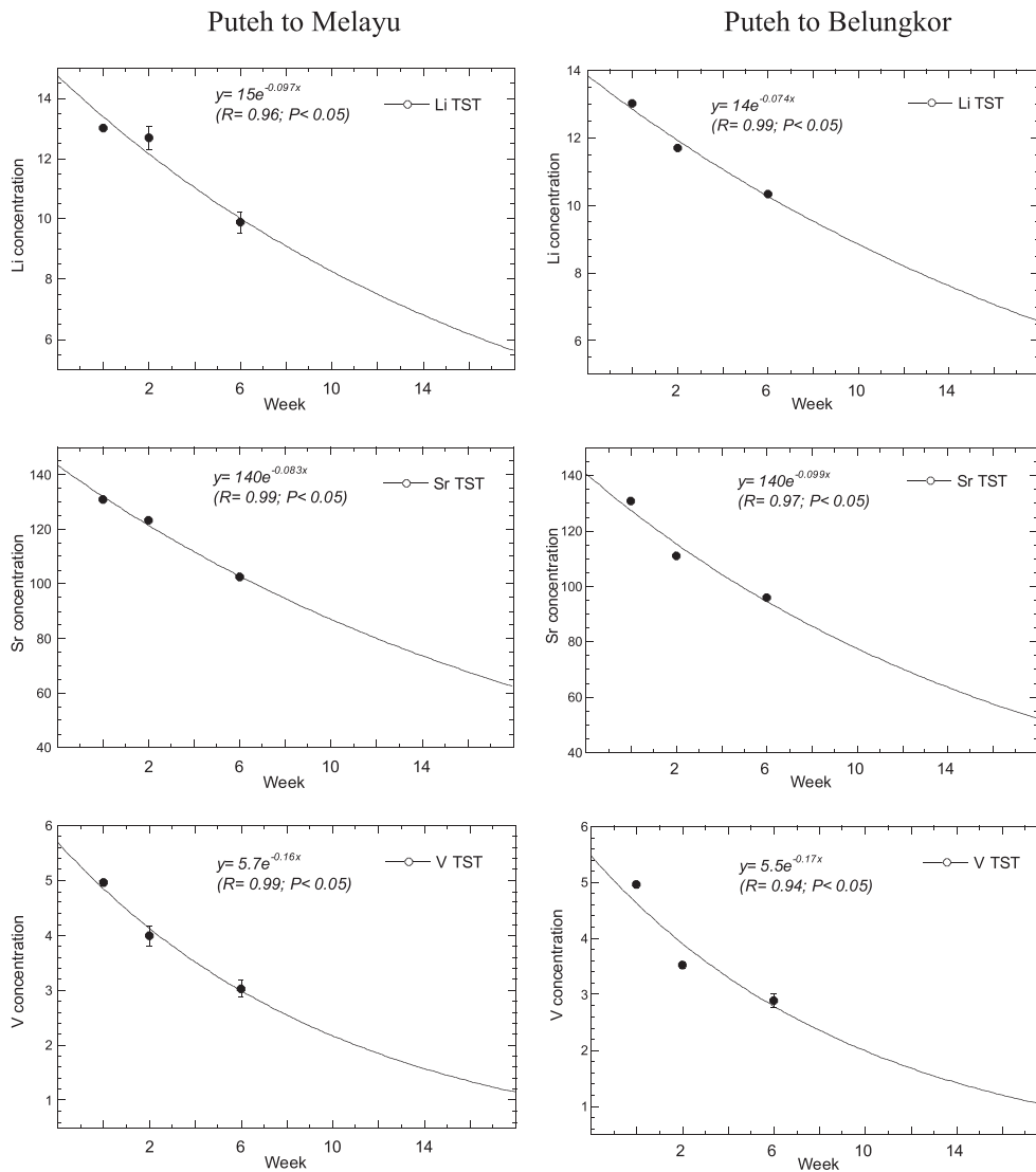
Fig. 2. Li, Sr, and V concentrations (mg/kg dry weight) in the mussels Perna viridis transplanted from Kg. Pasir Puteh to Kg. Sungai Melayu (Puteh to Melayu; left) and to Sungai Belungkor (Puteh to Belungkor; right). Curve fits are based on exponential equations.
