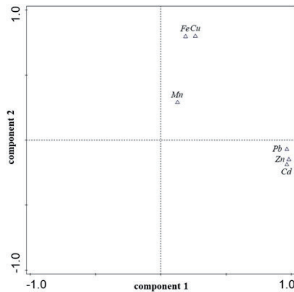
Fig. 4. Principal component analysis diagram of Caohai surface sediment.
