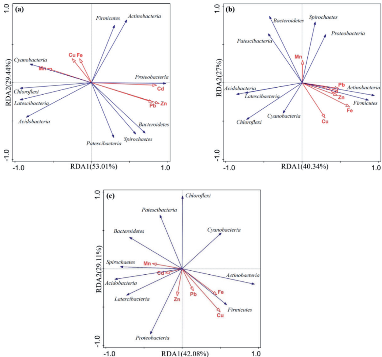
Fig. 13. RDA analysis of the relationship between Caohai sediment microbial communities and heavy metals in three regions.
