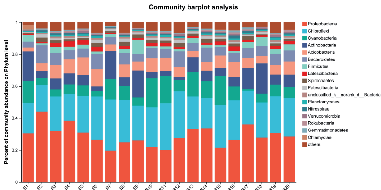
Fig. 10. Composition of bacterial species at each sampling point at the Phylum level.
