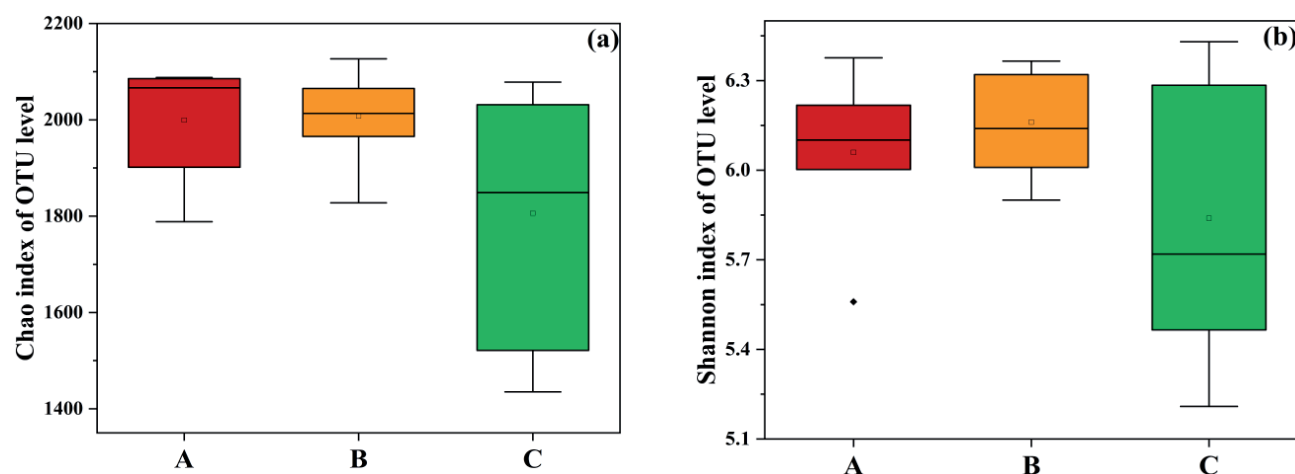
Fig. 9. \alpha diversity index of microbial communities in A, B, and C regions in Caohai sediment samples.
