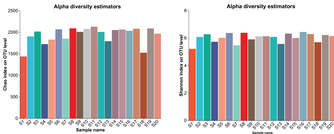
Fig. 8. Microbial community \alpha diversity index in Caohai sediment samples.
