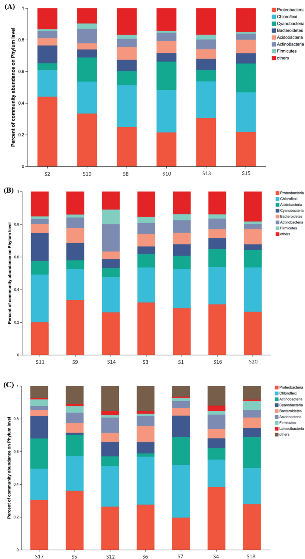
Fig. 11. Composition of bacterial species in areas A, B, and C at phyla level.
