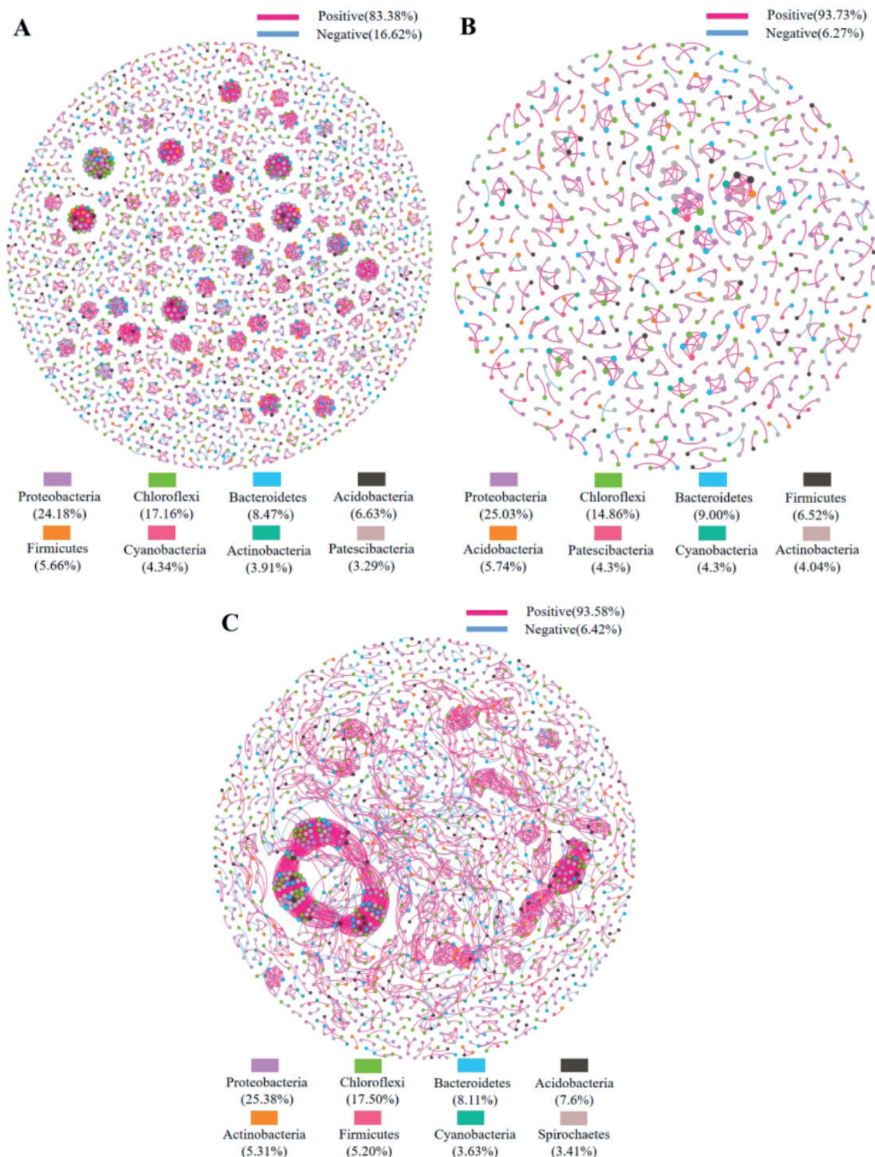
A, B, and C are co-occurrence networks of heavily polluted, moderately polluted, and lightly polluted areas in the Caohai wetland, respectively. Nodes are colored according to gate horizontal abundance, and the edge is strongly correlated (Spearman R > |0.6| ), which is significant ( P < 0.05 ). The red line indicates positive interactions. The blue lines represent negative interactions.
