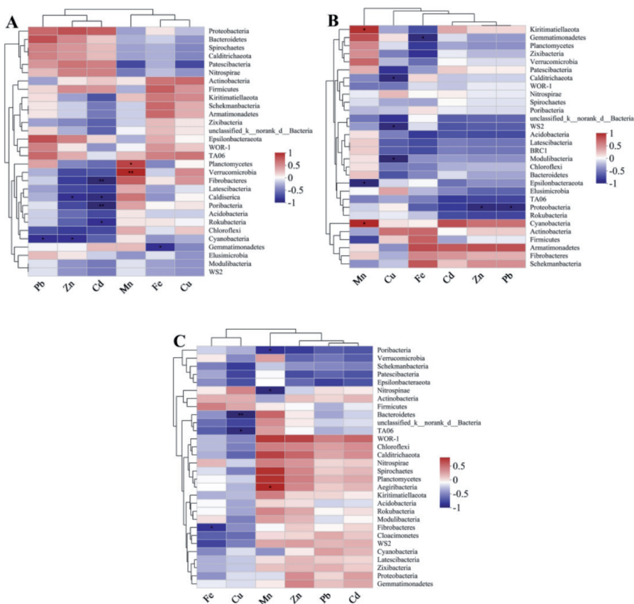
A, B, and C are the correlation heat maps of the heavily polluted area, moderately polluted area, and lightly polluted area of Caohai Wetland respectively. The color column indicates the correlation degree between bacterial community and heavy metals. If the correlation between the two is positive, it is shown in red; otherwise, if it is negative, it is shown in blue. The depth of the color indicates the strength of the correlation, and the darker the red, the higher the degree of positive correlation; The darker the blue, the higher the degree of negative correlation
