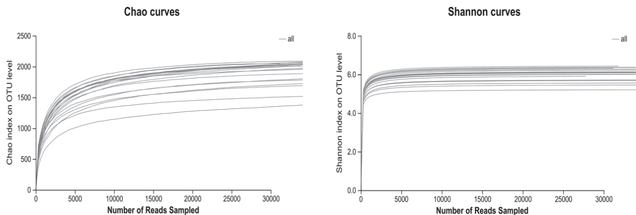
Fig. 7. Shannon and Chao index dilution curves of Caohai sediment samples.
