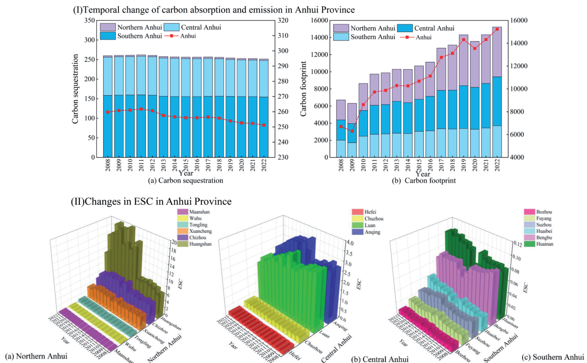
Fig. 2. Temporal and spatial variation of ESC in Anhui province.
