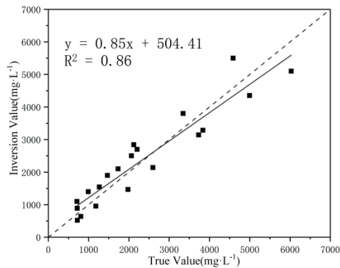
(e) BO-RF
