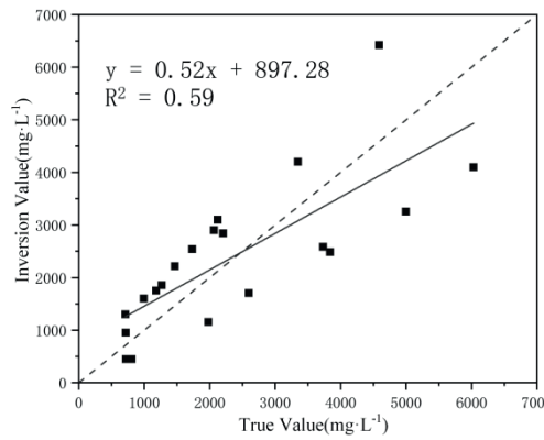
(a) SVR
