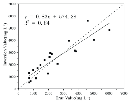
(c) XGBoost
