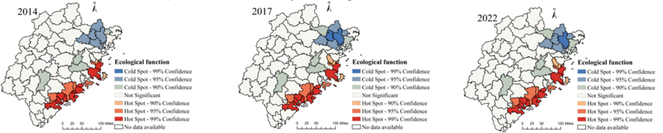
Fig. 2. Cold hotspot distribution in Fujian Province.
