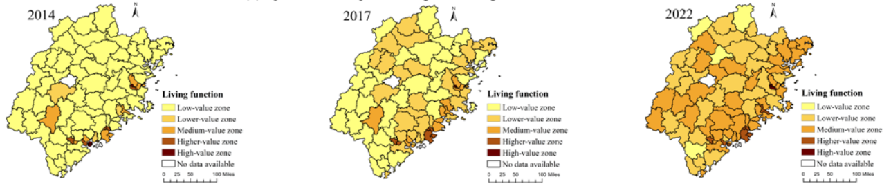
(b) Spatial and temporal changes in living function
