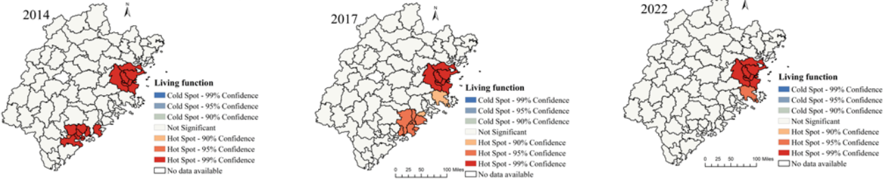
(c) Identification of cold/hot spots of ecological function
