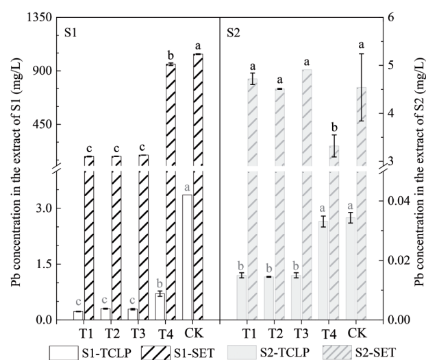
Fig. 1. TCLP extractable Pb and SET extractable Pb in two soils after the application of different amendments. Abbreviations are explained in Table 2.
