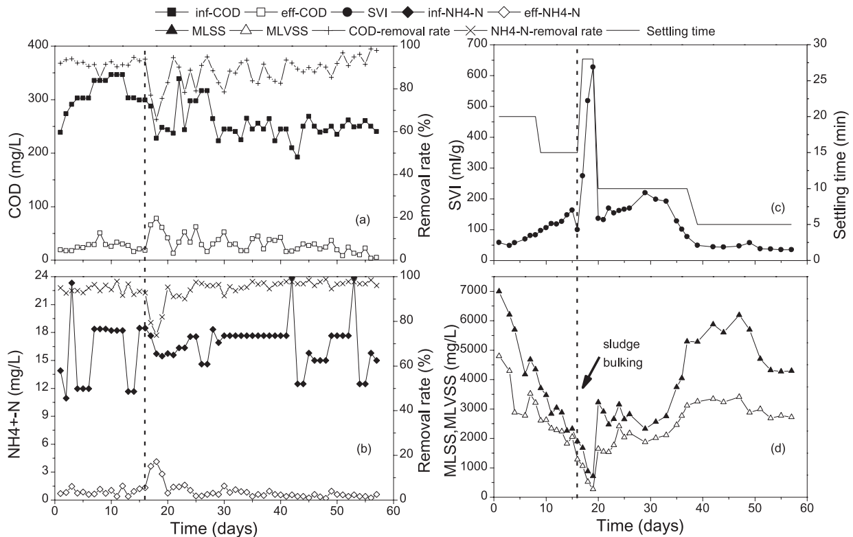
Fig. 1. Performance of the SBR system in the aerobic granulation stage.
