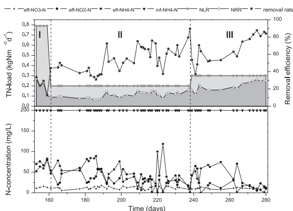
Fig. 5. Variation of nitrogen loading rate (NLR), nitrogen removal rate (NRR), removal efficiency, and N concentration of the autotrophic nitrogen removal process.
