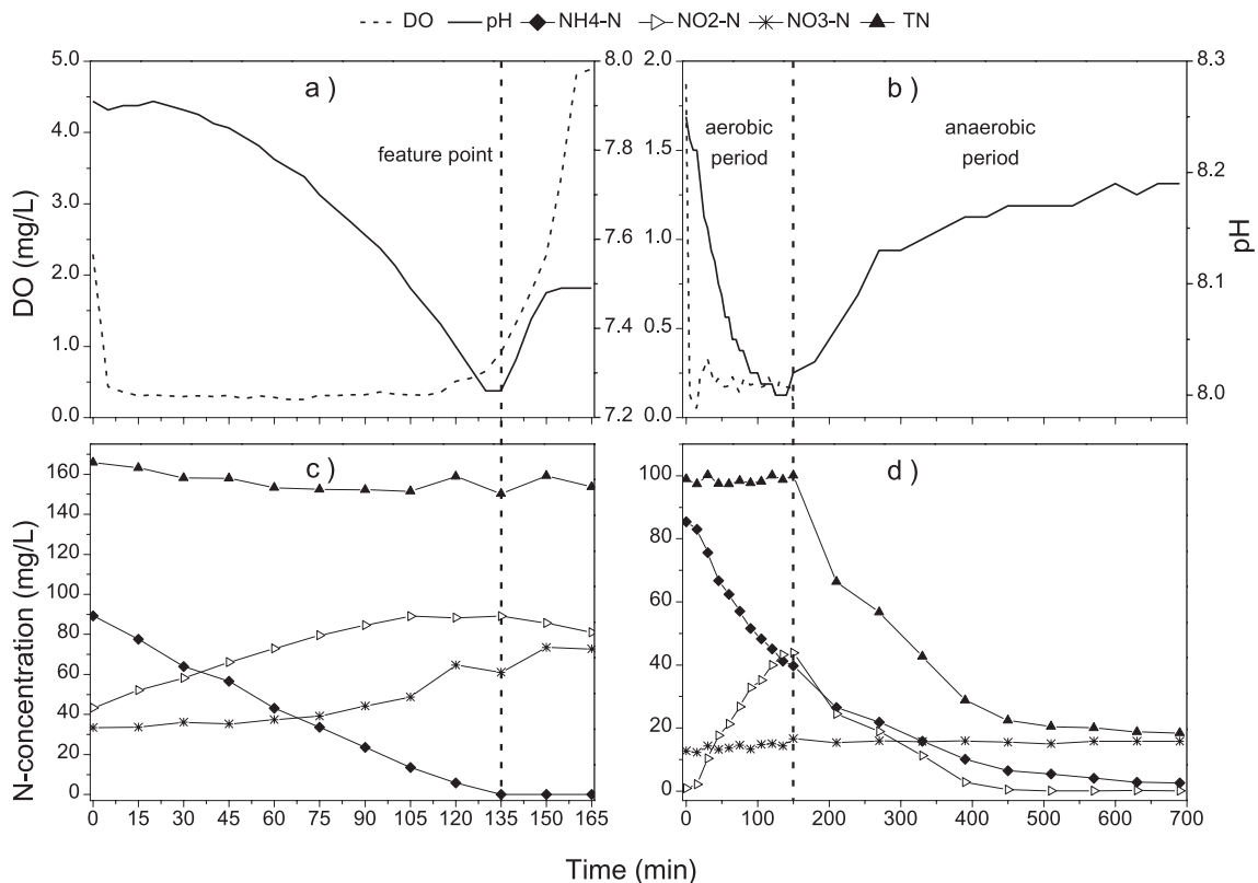
Fig. 4. Time course of parameters and substrates measured in two experimental phases: (a-c) nitrification regulation and (b-d) autotrophic nitrogen removal.
