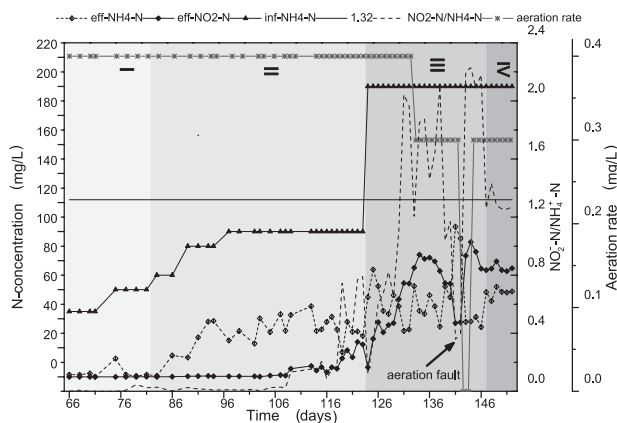
Fig. 3. Variations in influent/effluent concentrations of \text{NH}_4^+\text{-N} , \text{NO}_2^-\text{-N} , \text{NO}_2^-\text{-N}/\text{NH}_4^+\text{-N} and aeration rate in the nitritation process.
