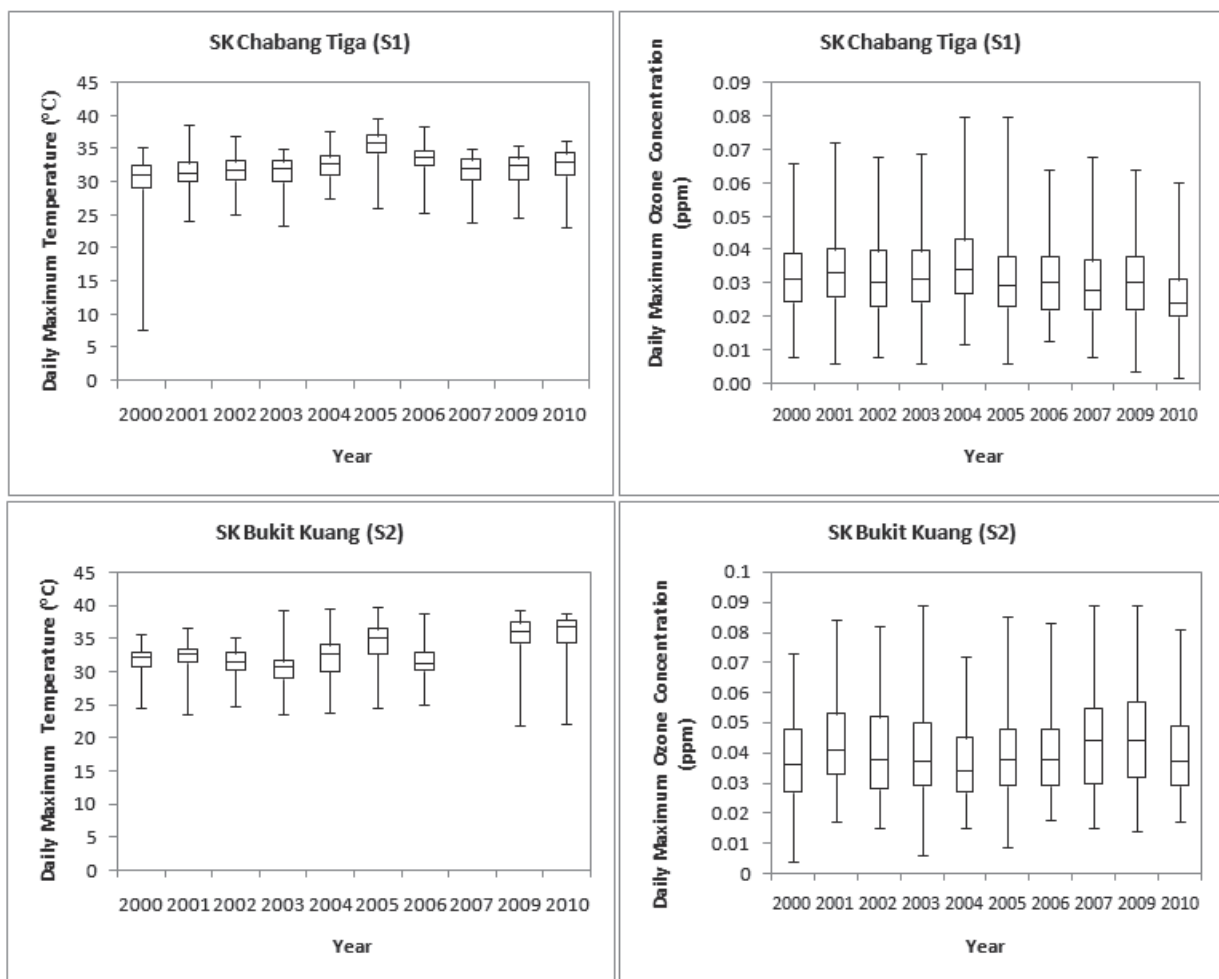
Fig. 2. The boxplot of daily maximum temperature and daily maximum ozone concentration trends for the period of 2000-2010*, *excluding year 2008.
