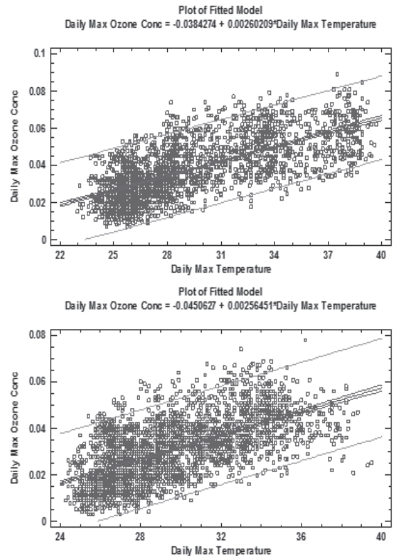
Fig. 4. Scatter plots of daily maximum temperature and daily maximum ozone concentration for the period of 2000-2010*, *excluding year 2008.
