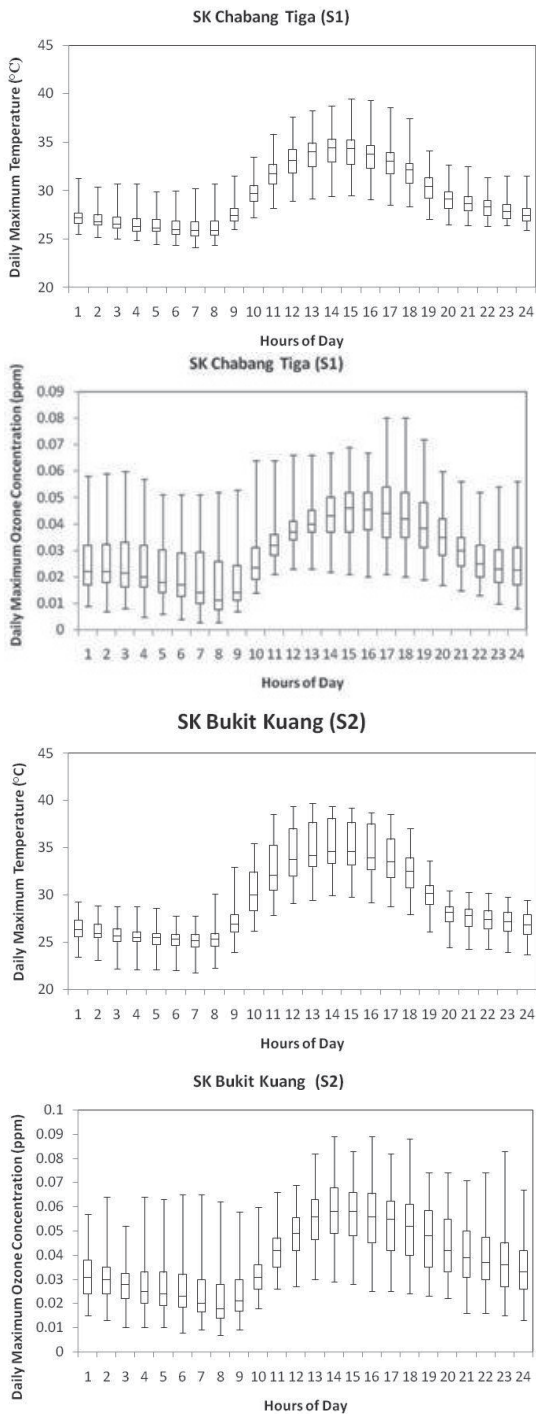
Fig. 3. Boxplot of the diurnal variations of daily maximum temperature and daily maximum ozone concentration for the period of 2000-2010*, *excluding year 2008.
