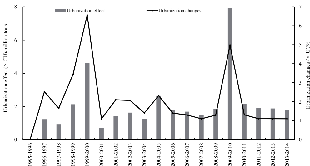
Fig. 2. Urbanization effect and urbanization changes from 1995 to 2014.
