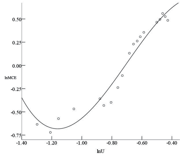
Fig. 3. Fit curve of marginal urbanization effect and urbanization.
