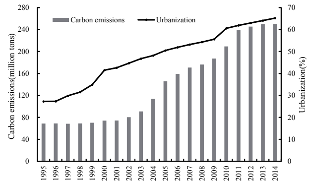
Fig. 1. The evolution process of energy-related carbon emissions and urbanization.
