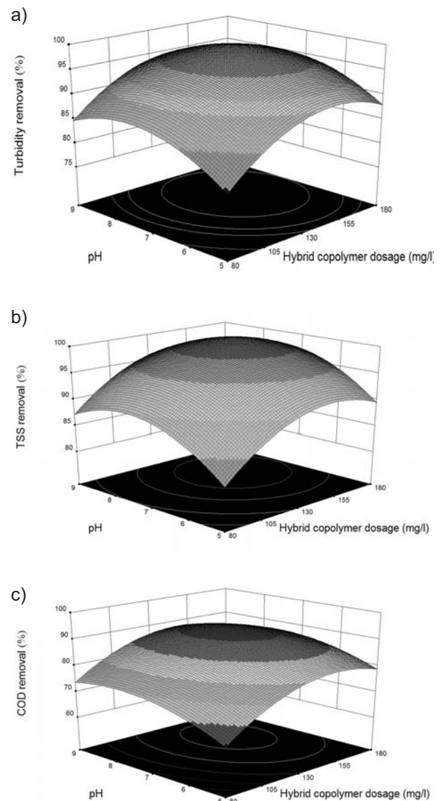
Fig. 4. 3D surface plot for (a) turbidity removal, (b) TSS removal, and (c) COD removal.
