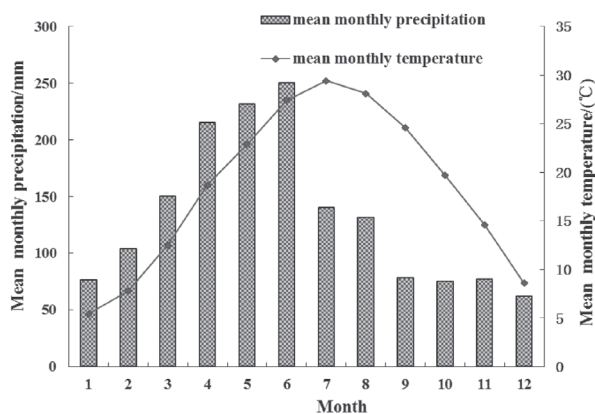
Fig. 3. Mean monthly precipitation and temperature in the study area (1971-2013 year).
