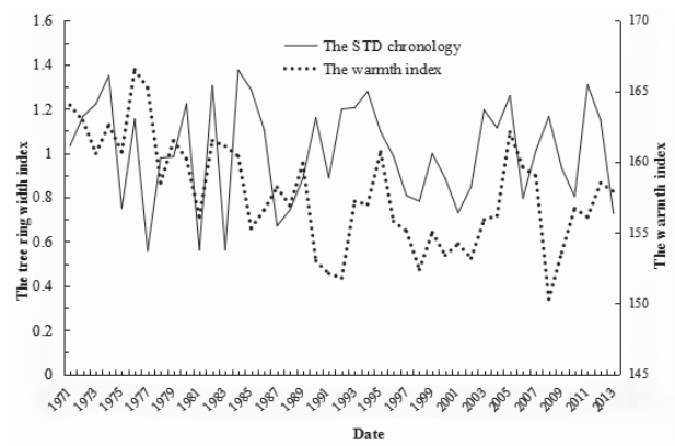
Fig. 6. Trend of the tree ring width index and the warmth index.
