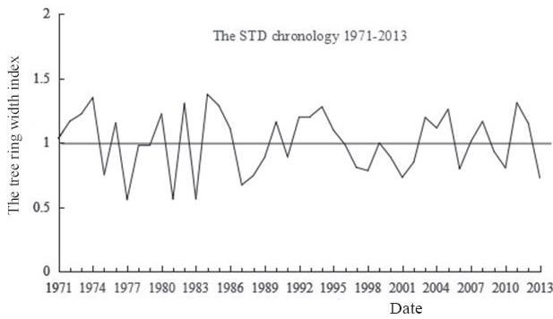
Fig. 4. Standard chronology from Chinese fir tree ring width.
