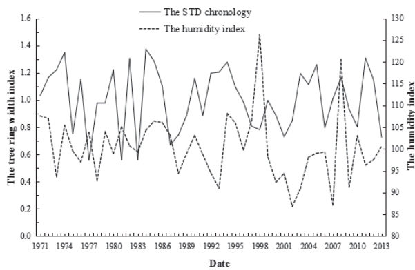
Fig. 8. Trend of the tree ring width index and the humidity index.
