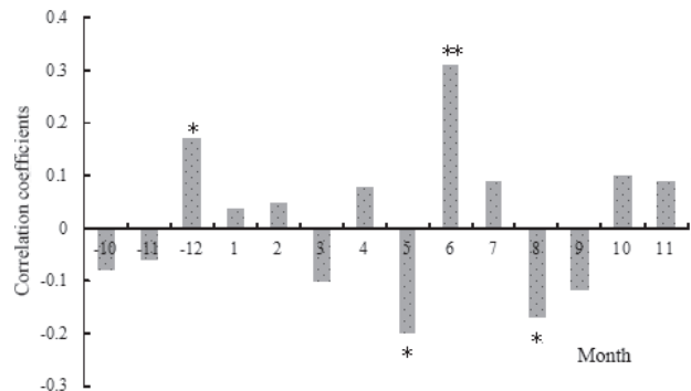
Fig. 7. Correlation coefficients between tree ring width and mean monthly precipitation. Note: * is p < 0.05 , ** is p < 0.01 .
