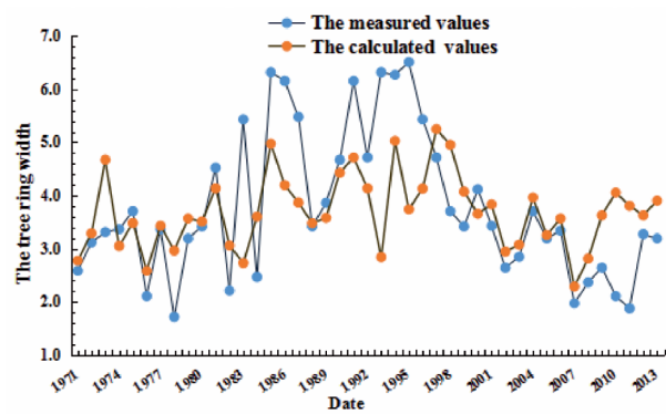
Fig. 9. Trend of the modeled ring width values and the measured values.
