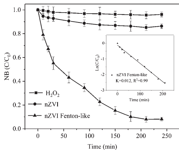
Fig. 2. Removal curves of NB in \text{H}_2\text{O}_2 , nZVI, and nZVI Fenton-like systems; inset graph is the plots of \ln(C/C_0) versus time for the removal of NB in an nZVI Fenton-like system.
